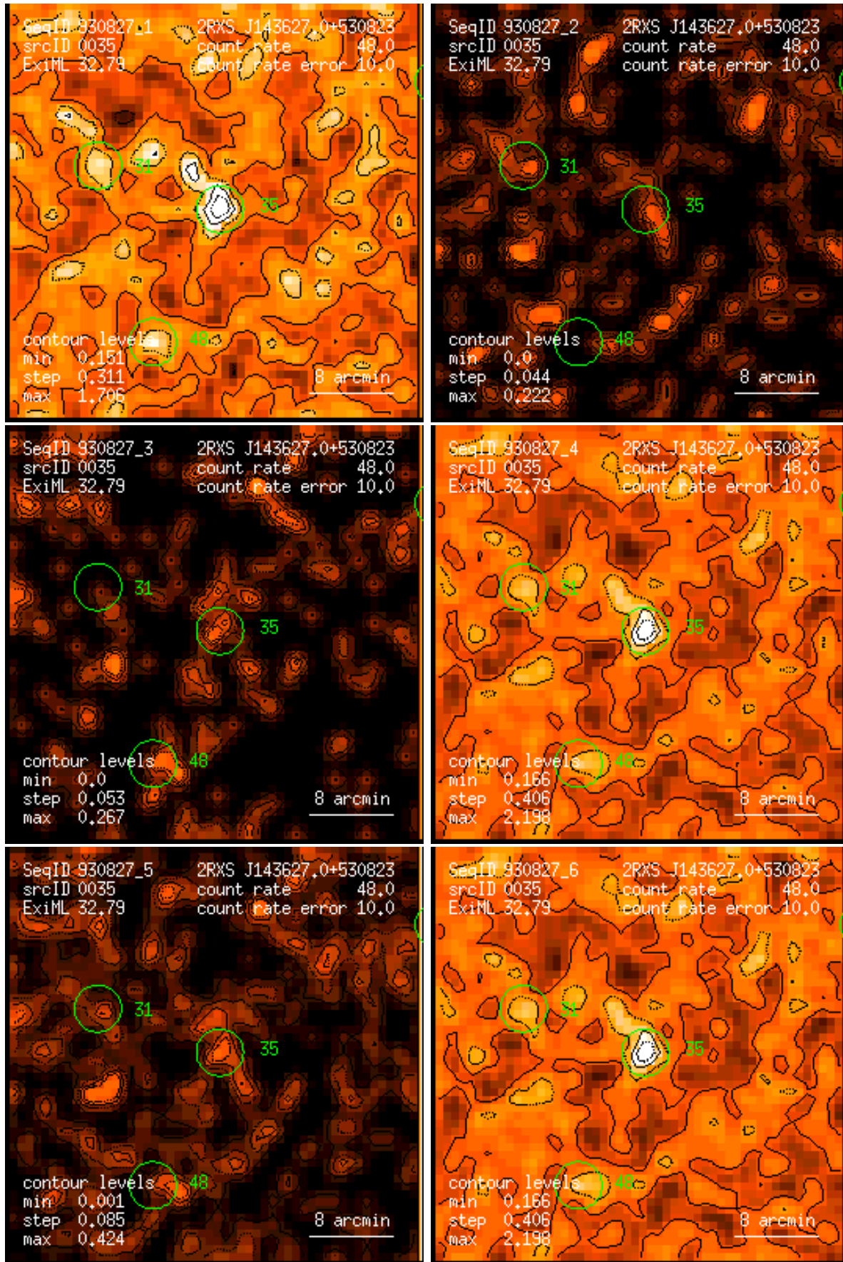
Figure 35: RASS 930827: detection 0035: band rate images, Gaussian filter: (1) PSPC channels 11 – 41, (2) 52 – 90, (3) 91 – 201, (4) 11 – 235, (5) 52 – 201, (6) 11 – 201. Broad band rates in counts/ks. Band rate contour levels in counts/ks/arcmin 2 .
