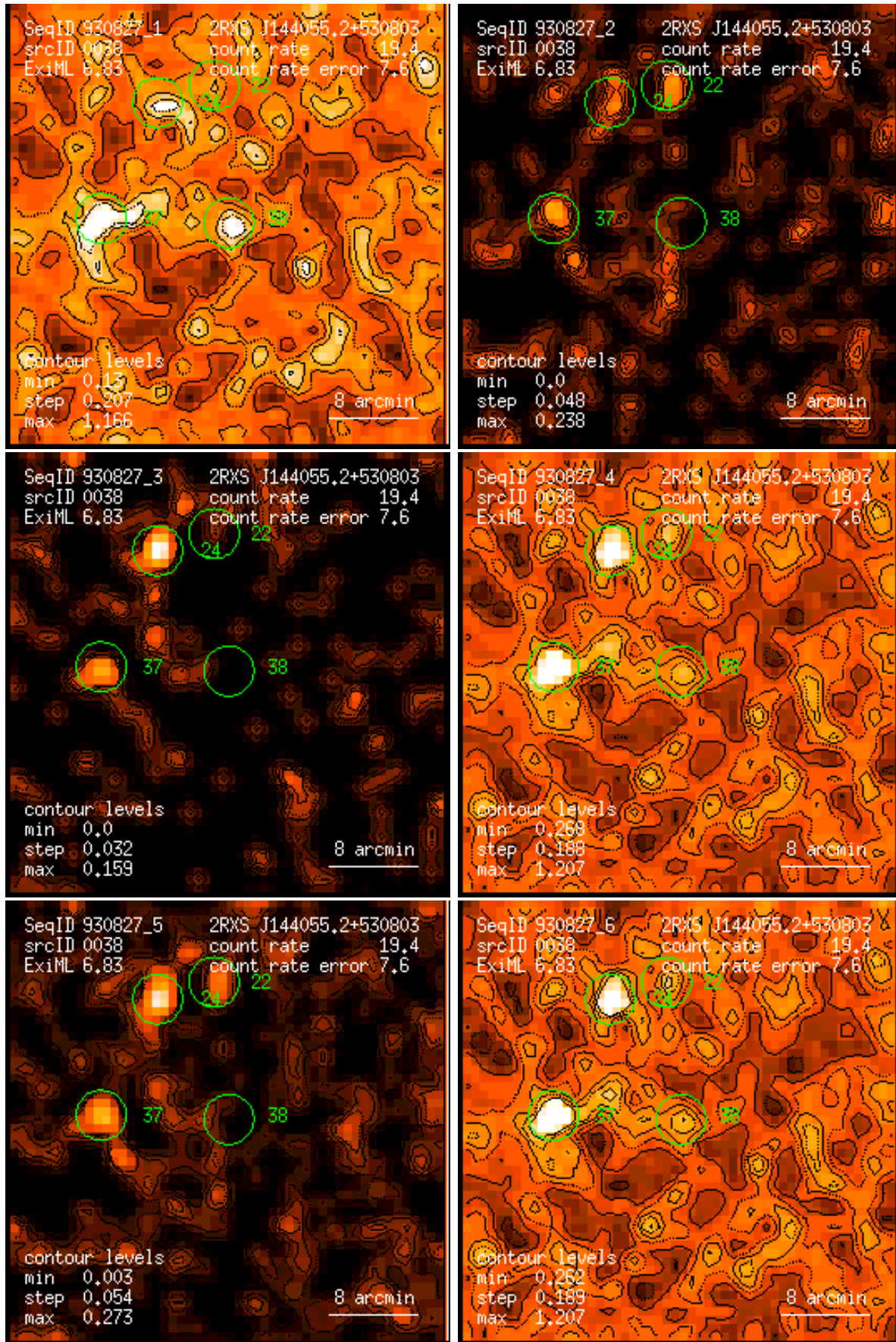
Figure 38: RASS 930827: detection 0038: band rate images, Gaussian filter: (1) PSPC channels 11 – 41, (2) 52 – 90, (3) 91 – 201, (4) 11 – 235, (5) 52 – 201, (6) 11 – 201. Broad band rates in counts/ks. Band rate contour levels in counts/ks/arcmin 2 .
