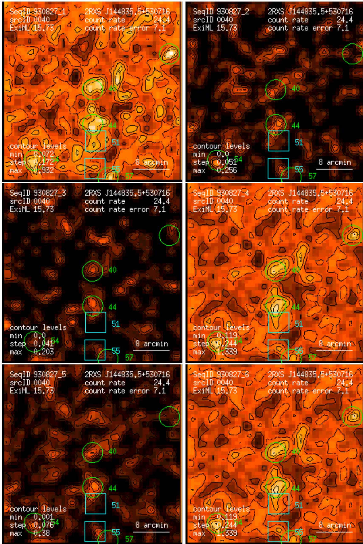
Figure 40: RASS 930827: detection 0040: band rate images, Gaussian filter: (1) PSPC channels 11 – 41, (2) 52 – 90, (3) 91 – 201, (4) 11 – 235, (5) 52 – 201, (6) 11 – 201. Broad band rates in counts/ks. Band rate contour levels in counts/ks/arcmin 2 .
