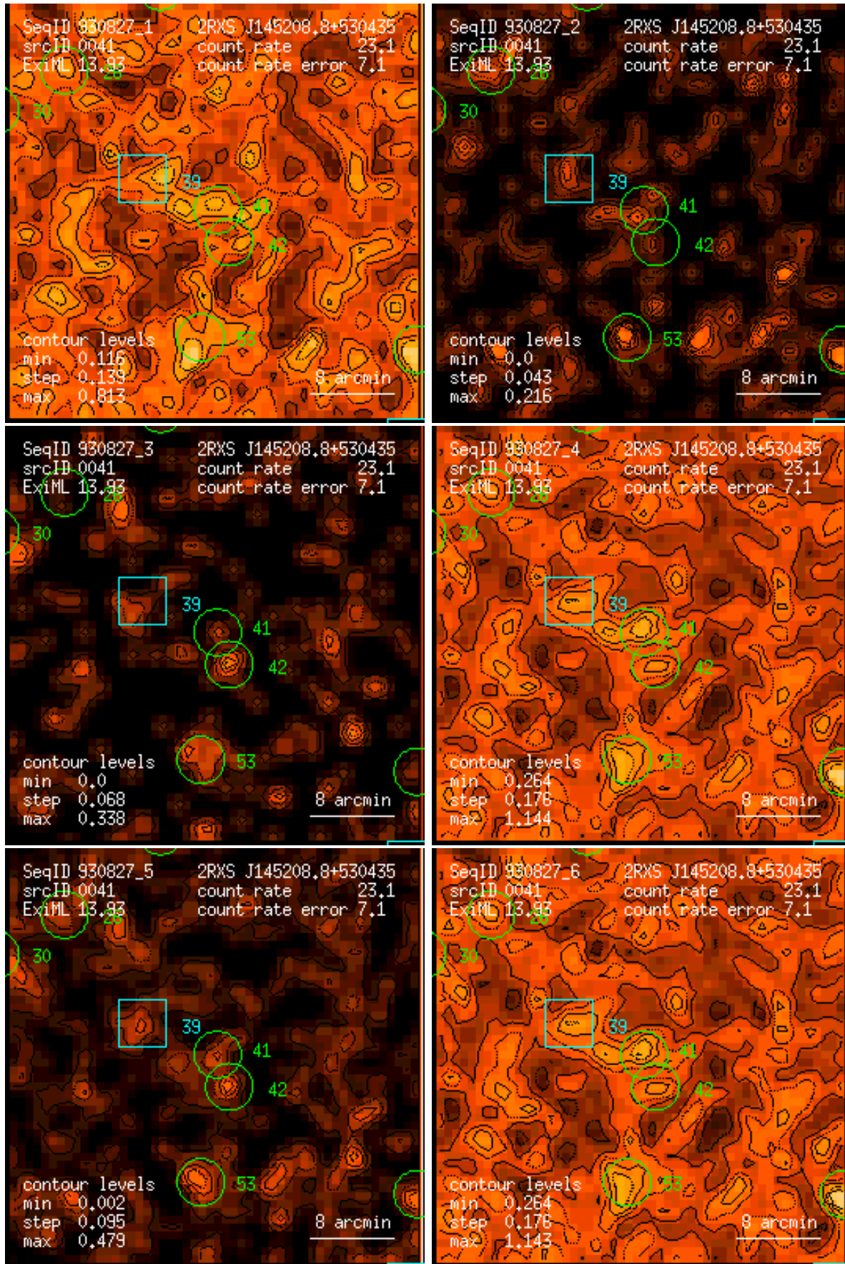
Figure 41: RASS 930827: detection 0041: band rate images, Gaussian filter: (1) PSPC channels 11 – 41, (2) 52 – 90, (3) 91 – 201, (4) 11 – 235, (5) 52 – 201, (6) 11 – 201. Broad band rates in counts/ks. Band rate contour levels in counts/ks/arcmin 2 .
