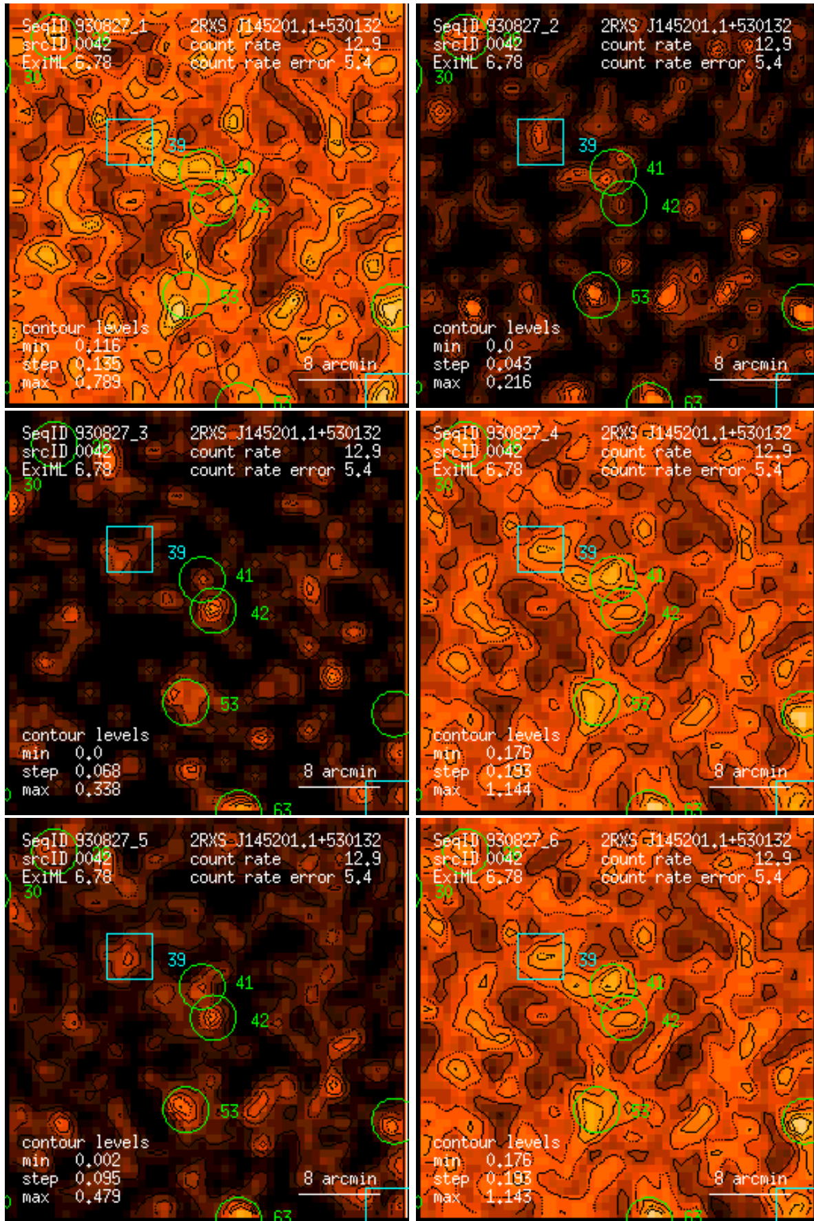
Figure 42: RASS 930827: detection 0042: band rate images, Gaussian filter: (1) PSPC channels 11 – 41, (2) 52 – 90, (3) 91 – 201, (4) 11 – 235, (5) 52 – 201, (6) 11 – 201. Broad band rates in counts/ks. Band rate contour levels in counts/ks/arcmin 2 .
