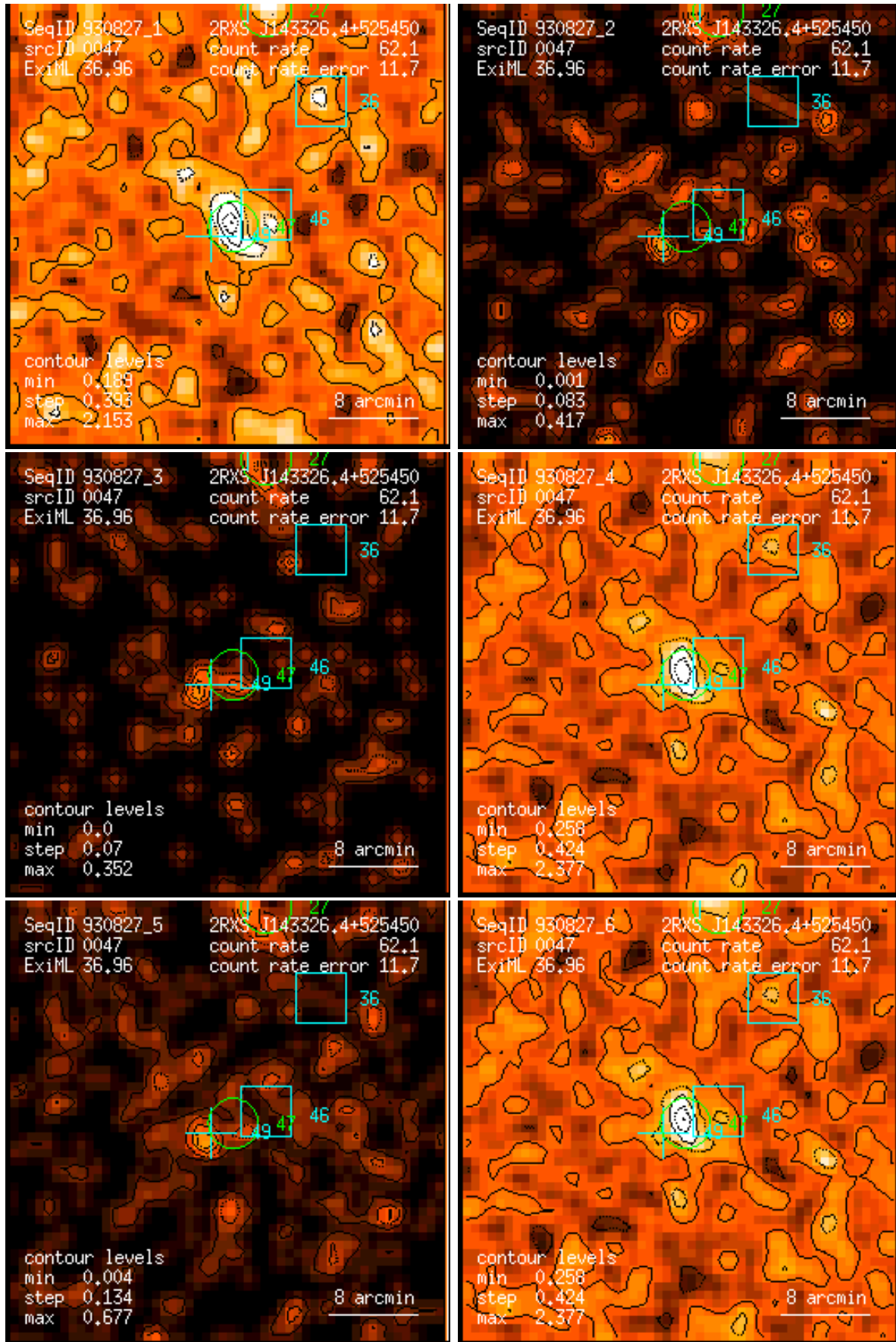
Figure 47: RASS 930827: detection 0047: band rate images, Gaussian filter: (1) PSPC channels 11 – 41, (2) 52 – 90, (3) 91 – 201, (4) 11 – 235, (5) 52 – 201, (6) 11 – 201. Broad band rates in counts/ks. Band rate contour levels in counts/ks/arcmin 2 .
