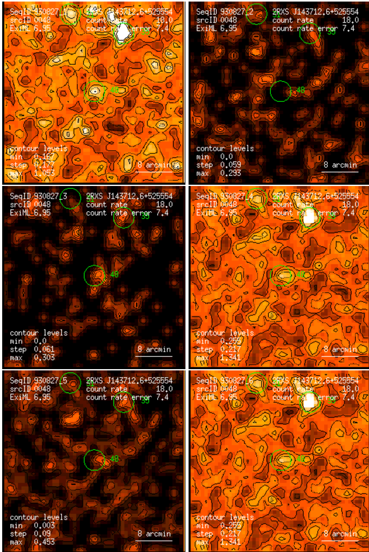
Figure 48: RASS 930827: detection 0048: band rate images, Gaussian filter: (1) PSPC channels 11 – 41, (2) 52 – 90, (3) 91 – 201, (4) 11 – 235, (5) 52 – 201, (6) 11 – 201. Broad band rates in counts/ks. Band rate contour levels in counts/ks/arcmin 2 .
