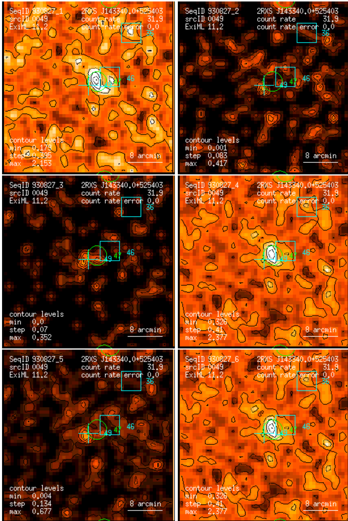
Figure 49: RASS 930827: detection 0049: band rate images, Gaussian filter: (1) PSPC channels 11 – 41, (2) 52 – 90, (3) 91 – 201, (4) 11 – 235, (5) 52 – 201, (6) 11 – 201. Broad band rates in counts/ks. Band rate contour levels in counts/ks/arcmin 2 .
