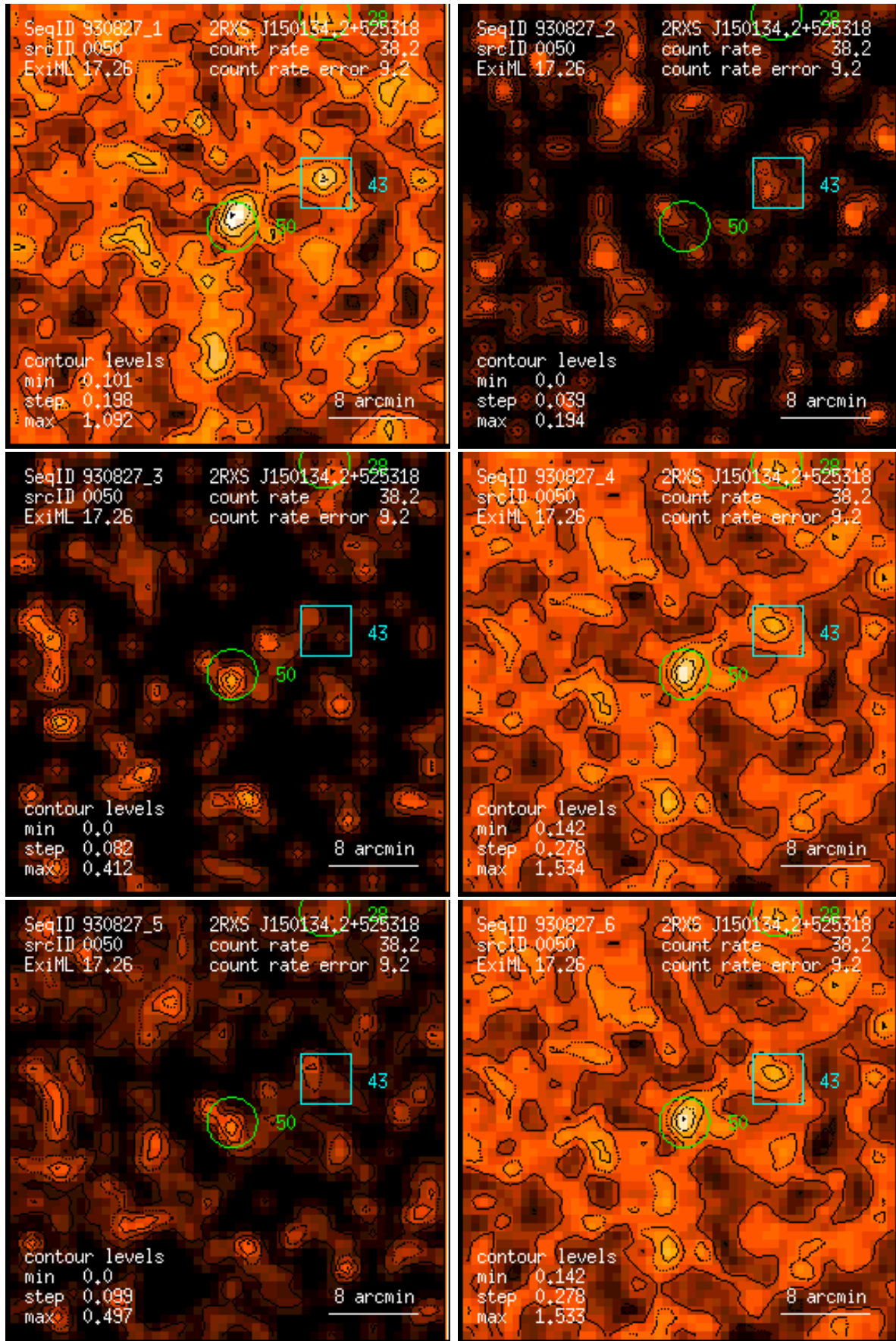
Figure 50: RASS 930827: detection 0050: band rate images, Gaussian filter: (1) PSPC channels 11 – 41, (2) 52 – 90, (3) 91 – 201, (4) 11 – 235, (5) 52 – 201, (6) 11 – 201. Broad band rates in counts/ks. Band rate contour levels in counts/ks/arcmin 2 .
