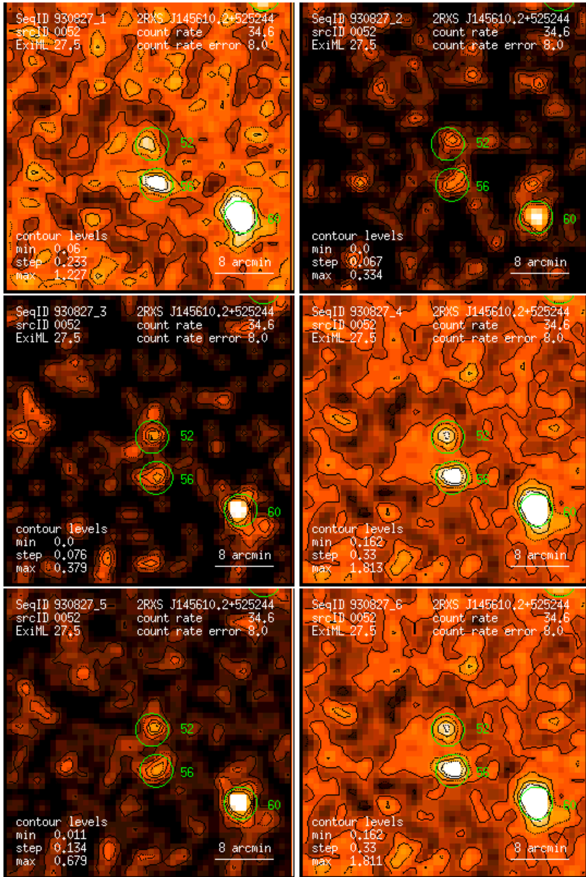
Figure 52: RASS 930827: detection 0052: band rate images, Gaussian filter: (1) PSPC channels 11 – 41, (2) 52 – 90, (3) 91 – 201, (4) 11 – 235, (5) 52 – 201, (6) 11 – 201. Broad band rates in counts/ks. Band rate contour levels in counts/ks/arcmin 2 .
