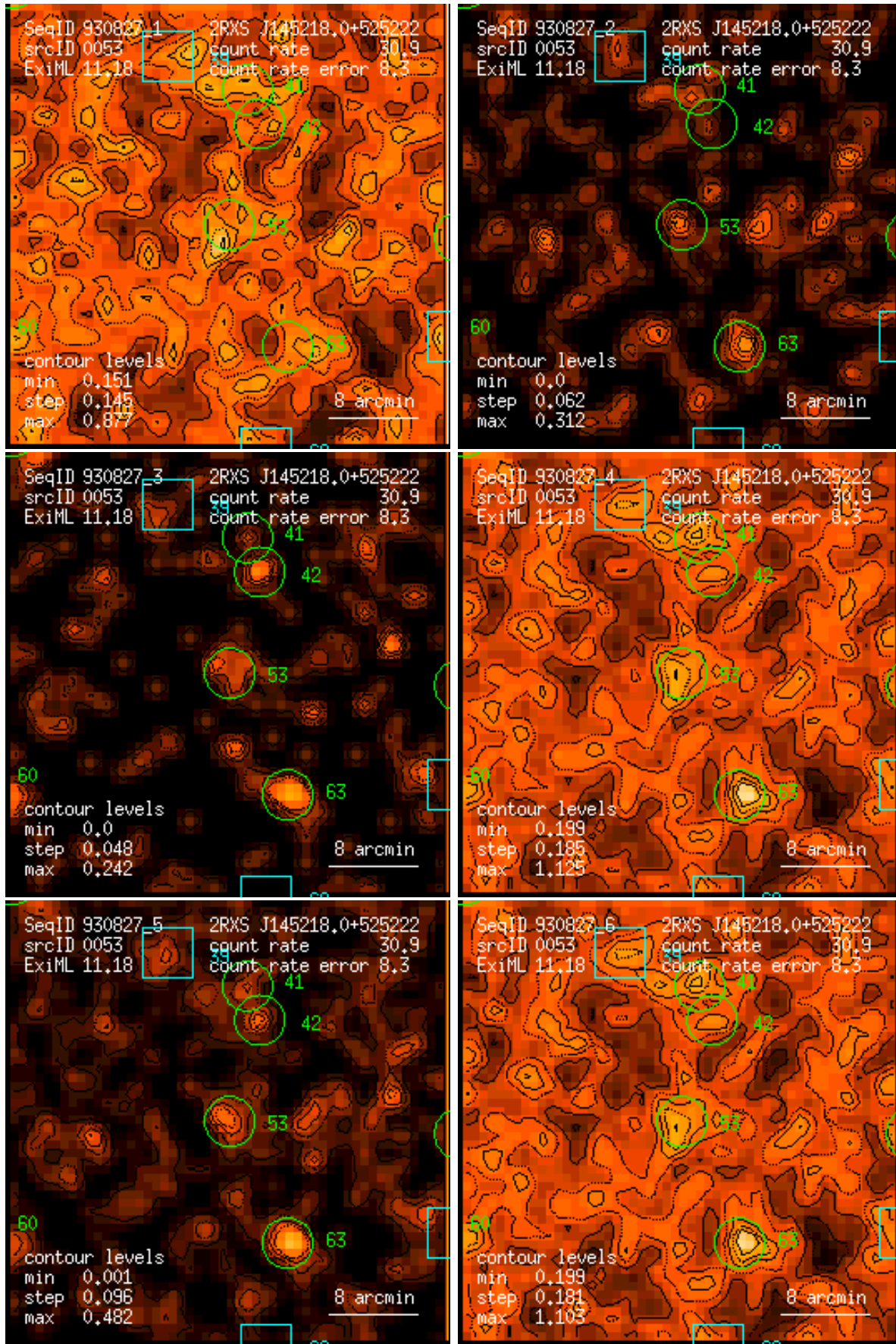
Figure 53: RASS 930827: detection 0053: band rate images, Gaussian filter: (1) PSPC channels 11 – 41, (2) 52 – 90, (3) 91 – 201, (4) 11 – 235, (5) 52 – 201, (6) 11 – 201. Broad band rates in counts/ks. Band rate contour levels in counts/ks/arcmin 2 .
