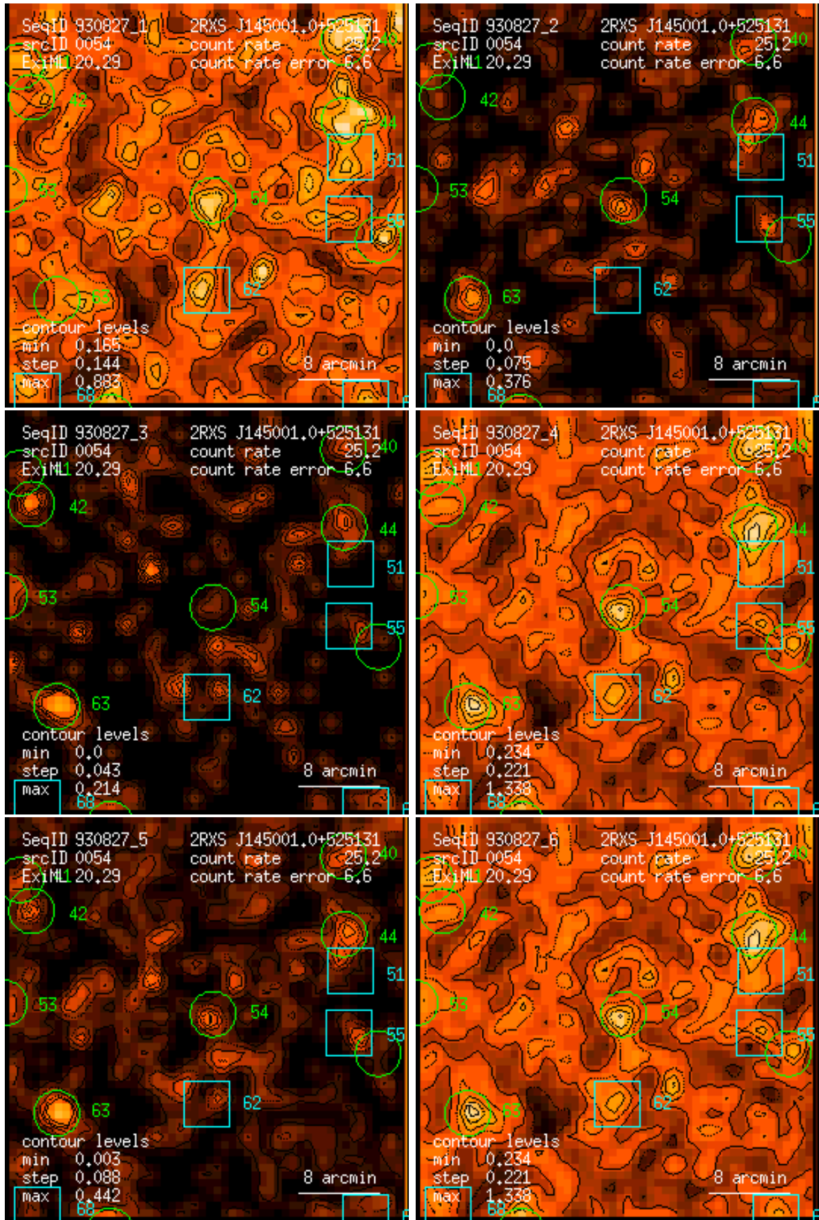
Figure 54: RASS 930827: detection 0054: band rate images, Gaussian filter: (1) PSPC channels 11 – 41, (2) 52 – 90, (3) 91 – 201, (4) 11 – 235, (5) 52 – 201, (6) 11 – 201. Broad band rates in counts/ks. Band rate contour levels in counts/ks/arcmin 2 .
