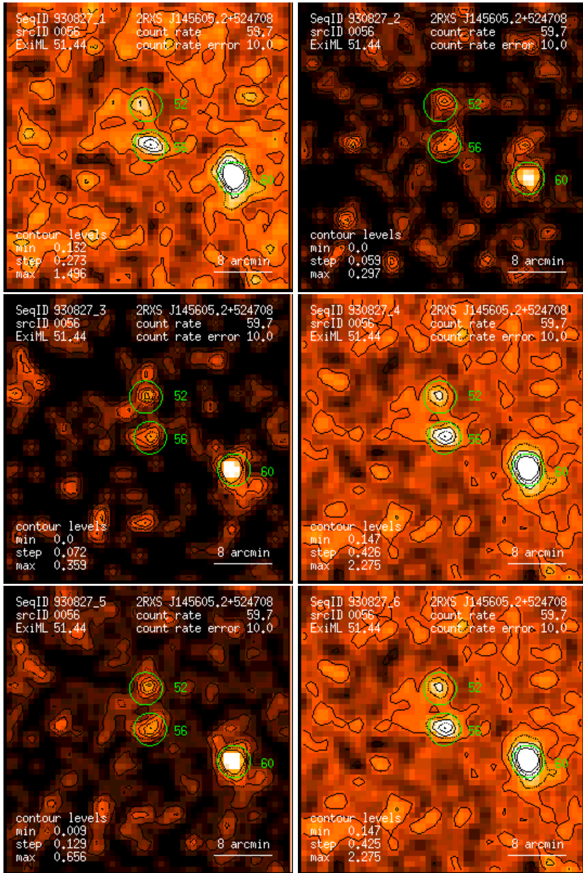
Figure 56: RASS 930827: detection 0056: band rate images, Gaussian filter: (1) PSPC channels 11 – 41, (2) 52 – 90, (3) 91 – 201, (4) 11 – 235, (5) 52 – 201, (6) 11 – 201. Broad band rates in counts/ks. Band rate contour levels in counts/ks/arcmin 2 .
