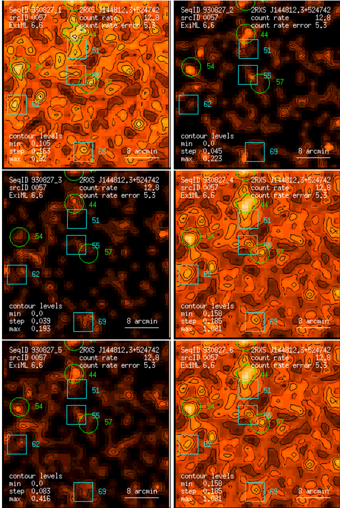
Figure 57: RASS 930827: detection 0057: band rate images, Gaussian filter: (1) PSPC channels 11 – 41, (2) 52 – 90, (3) 91 – 201, (4) 11 – 235, (5) 52 – 201, (6) 11 – 201. Broad band rates in counts/ks. Band rate contour levels in counts/ks/arcmin 2 .
