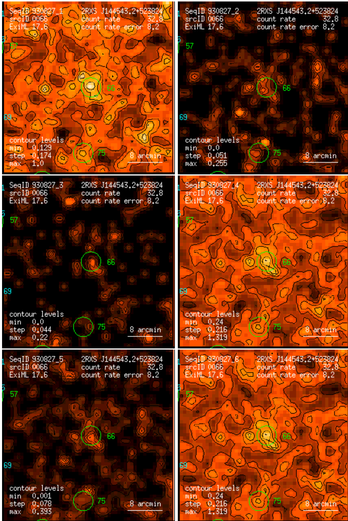
Figure 66: RASS 930827: detection 0066: band rate images, Gaussian filter: (1) PSPC channels 11 – 41, (2) 52 – 90, (3) 91 – 201, (4) 11 – 235, (5) 52 – 201, (6) 11 – 201. Broad band rates in counts/ks. Band rate contour levels in counts/ks/arcmin 2 .
