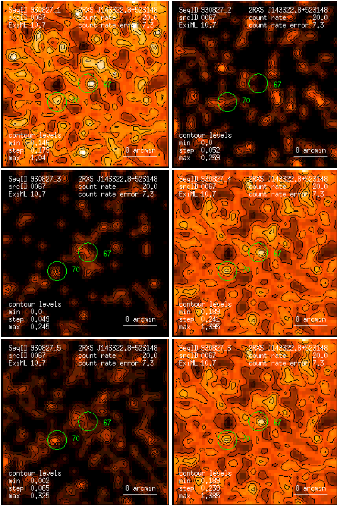
Figure 67: RASS 930827: detection 0067: band rate images, Gaussian filter: (1) PSPC channels 11 – 41, (2) 52 – 90, (3) 91 – 201, (4) 11 – 235, (5) 52 – 201, (6) 11 – 201. Broad band rates in counts/ks. Band rate contour levels in counts/ks/arcmin 2 .
