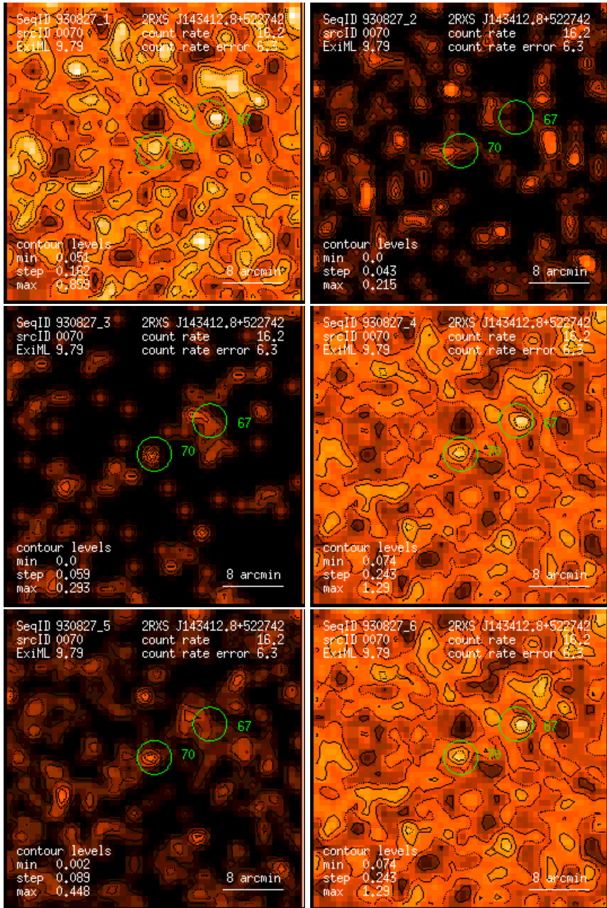
Figure 70: RASS 930827: detection 0070: band rate images, Gaussian filter: (1) PSPC channels 11 – 41, (2) 52 – 90, (3) 91 – 201, (4) 11 – 235, (5) 52 – 201, (6) 11 – 201. Broad band rates in counts/ks. Band rate contour levels in counts/ks/arcmin 2 .
