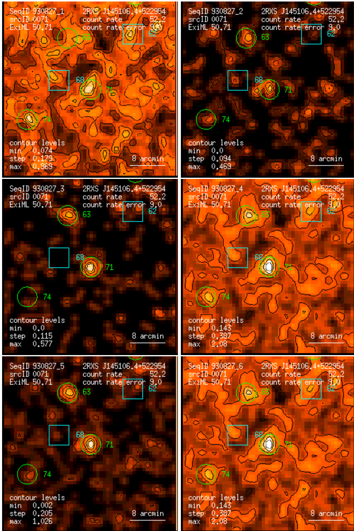
Figure 71: RASS 930827: detection 0071: band rate images, Gaussian filter: (1) PSPC channels 11 – 41, (2) 52 – 90, (3) 91 – 201, (4) 11 – 235, (5) 52 – 201, (6) 11 – 201. Broad band rates in counts/ks. Band rate contour levels in counts/ks/arcmin 2 .
