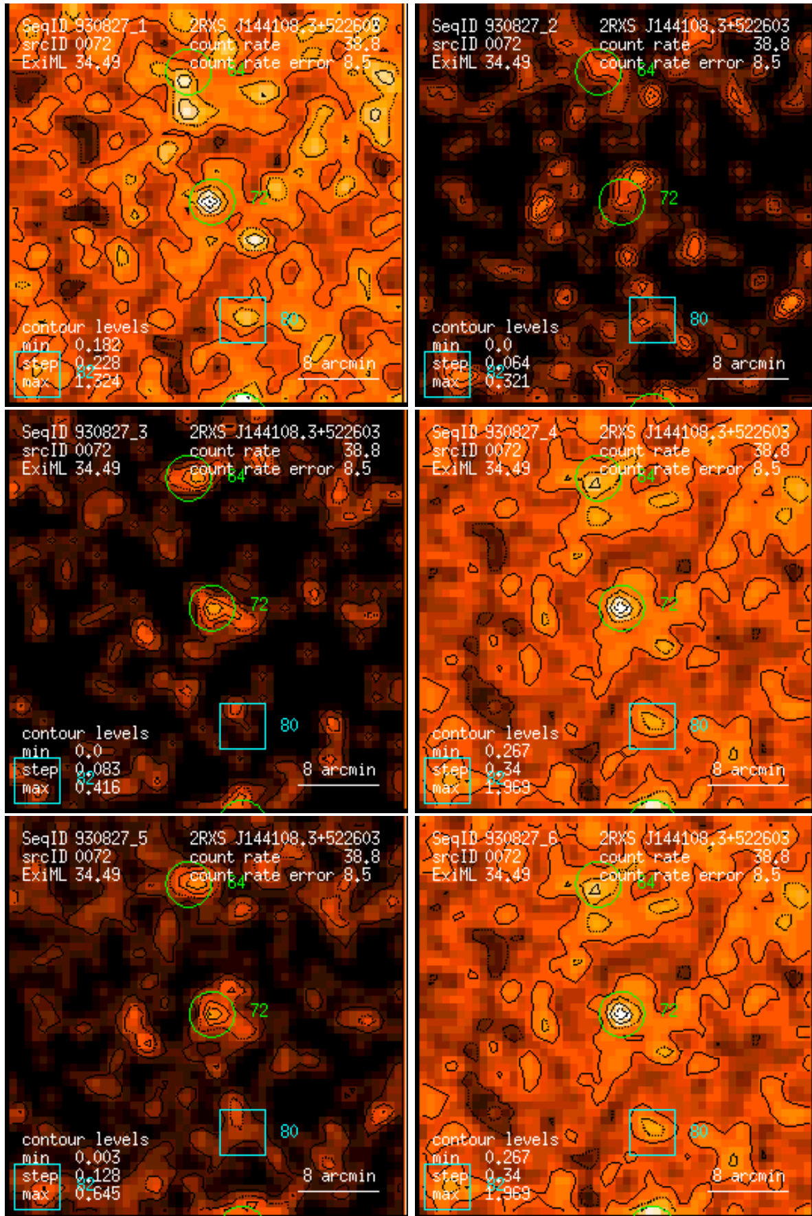
Figure 72: RASS 930827: detection 0072: band rate images, Gaussian filter: (1) PSPC channels 11 – 41, (2) 52 – 90, (3) 91 – 201, (4) 11 – 235, (5) 52 – 201, (6) 11 – 201. Broad band rates in counts/ks. Band rate contour levels in counts/ks/arcmin 2 .
