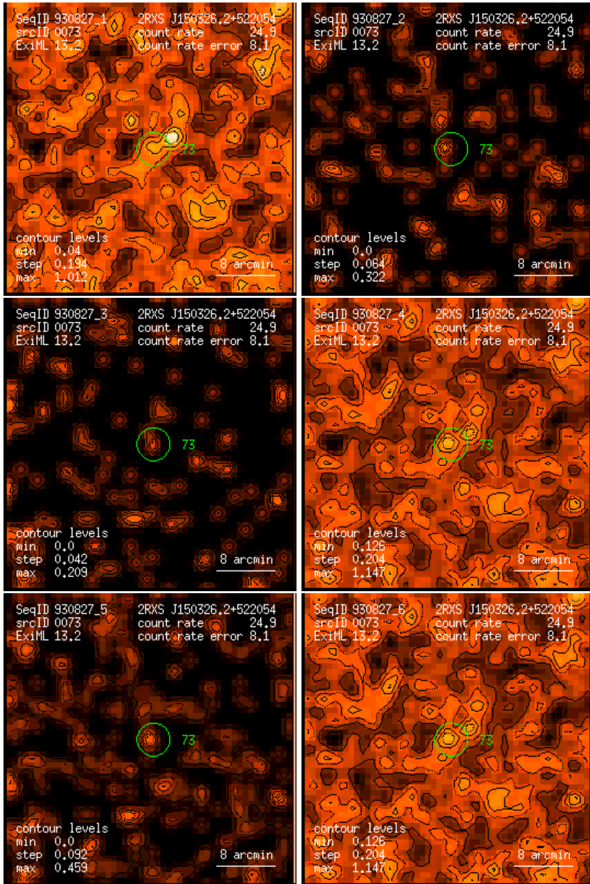
Figure 73: RASS 930827: detection 0073: band rate images, Gaussian filter: (1) PSPC channels 11 – 41, (2) 52 – 90, (3) 91 – 201, (4) 11 – 235, (5) 52 – 201, (6) 11 – 201. Broad band rates in counts/ks. Band rate contour levels in counts/ks/arcmin 2 .
