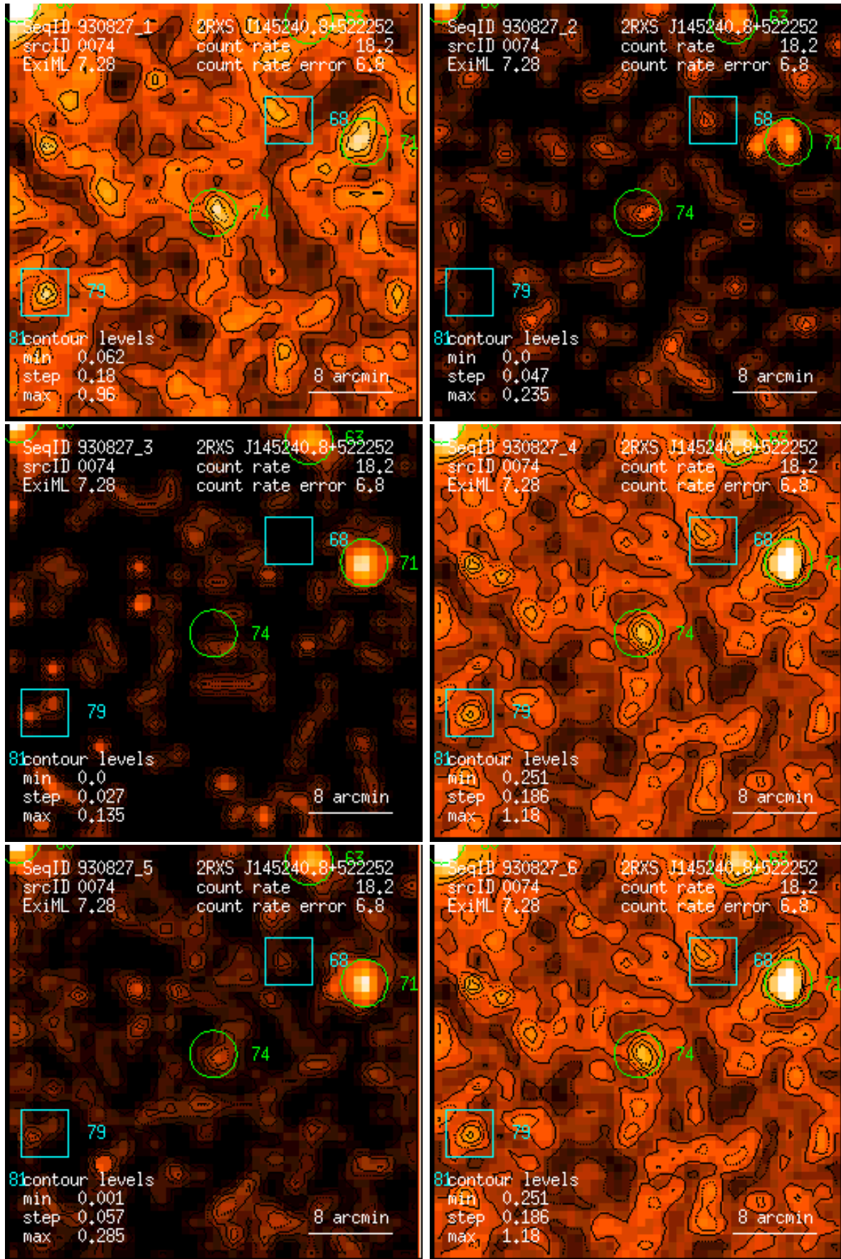
Figure 74: RASS 930827: detection 0074: band rate images, Gaussian filter: (1) PSPC channels 11 – 41, (2) 52 – 90, (3) 91 – 201, (4) 11 – 235, (5) 52 – 201, (6) 11 – 201. Broad band rates in counts/ks. Band rate contour levels in counts/ks/arcmin 2 .
