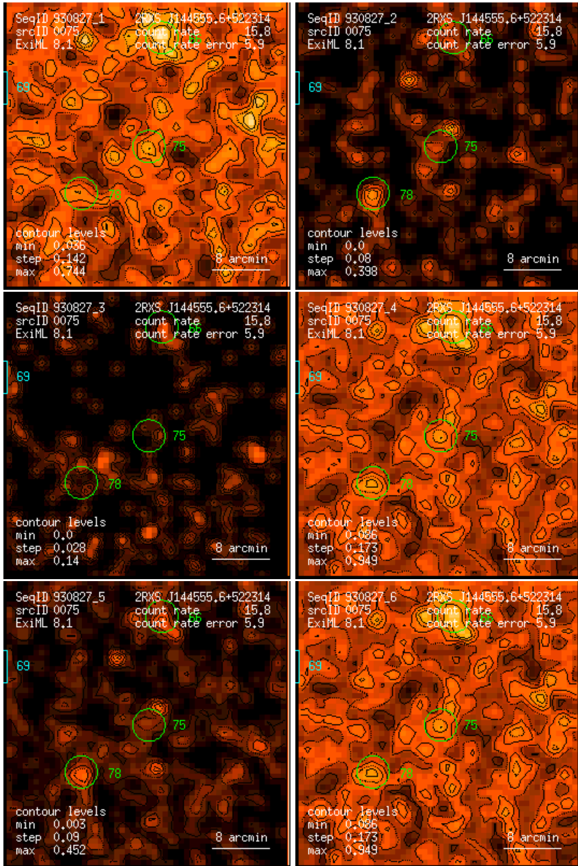
Figure 75: RASS 930827: detection 0075: band rate images, Gaussian filter: (1) PSPC channels 11 – 41, (2) 52 – 90, (3) 91 – 201, (4) 11 – 235, (5) 52 – 201, (6) 11 – 201. Broad band rates in counts/ks. Band rate contour levels in counts/ks/arcmin 2 .
