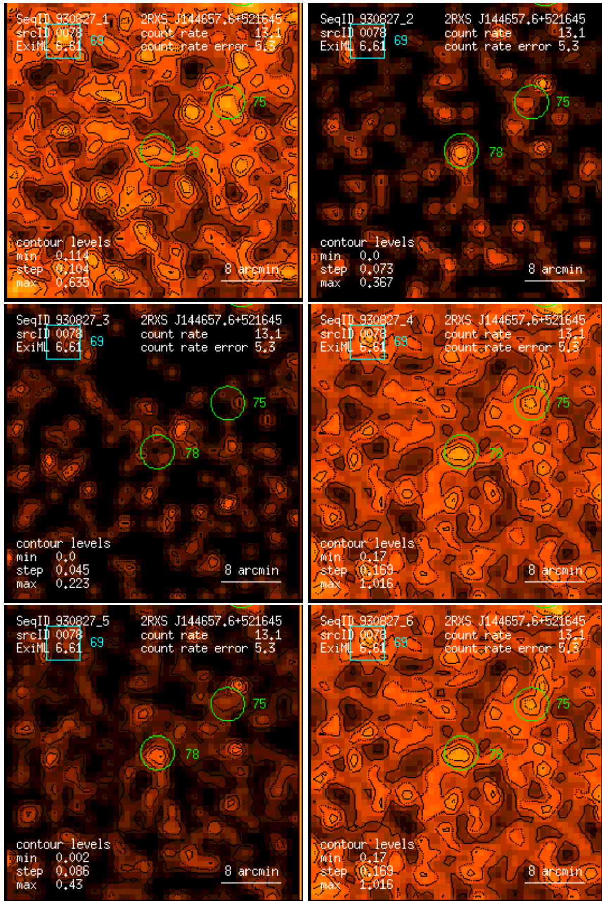
Figure 78: RASS 930827: detection 0078: band rate images, Gaussian filter: (1) PSPC channels 11 – 41, (2) 52 – 90, (3) 91 – 201, (4) 11 – 235, (5) 52 – 201, (6) 11 – 201. Broad band rates in counts/ks. Band rate contour levels in counts/ks/arcmin 2 .
