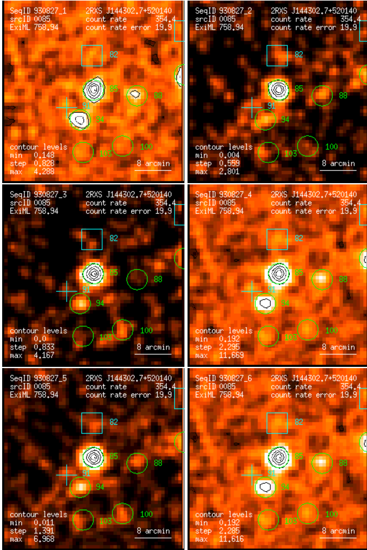
Figure 85: RASS 930827: detection 0085: band rate images, Gaussian filter: (1) PSPC channels 11 – 41, (2) 52 – 90, (3) 91 – 201, (4) 11 – 235, (5) 52 – 201, (6) 11 – 201. Broad band rates in counts/ks. Band rate contour levels in counts/ks/arcmin 2 .
