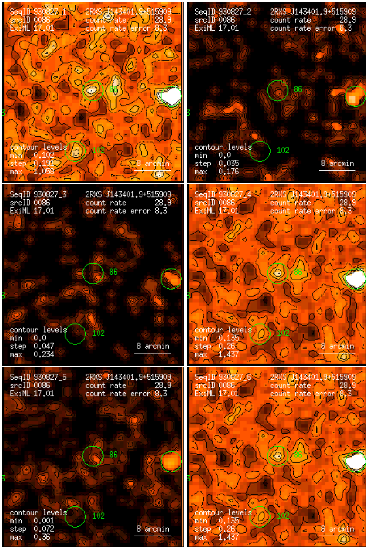
Figure 86: RASS 930827: detection 0086: band rate images, Gaussian filter: (1) PSPC channels 11 – 41, (2) 52 – 90, (3) 91 – 201, (4) 11 – 235, (5) 52 – 201, (6) 11 – 201. Broad band rates in counts/ks. Band rate contour levels in counts/ks/arcmin 2 .
