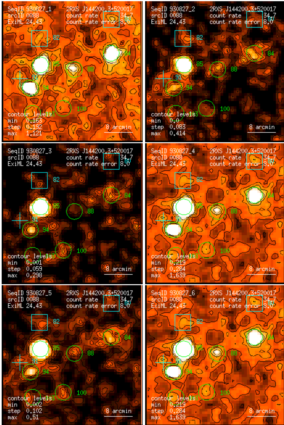
Figure 88: RASS 930827: detection 0088: band rate images, Gaussian filter: (1) PSPC channels 11 – 41, (2) 52 – 90, (3) 91 – 201, (4) 11 – 235, (5) 52 – 201, (6) 11 – 201. Broad band rates in counts/ks. Band rate contour levels in counts/ks/arcmin 2 .
