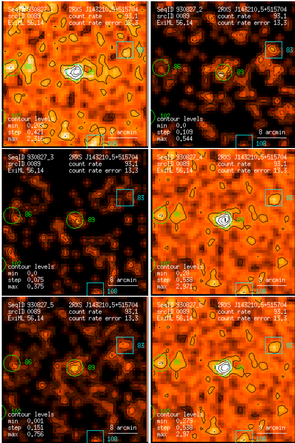
Figure 89: RASS 930827: detection 0089: band rate images, Gaussian filter: (1) PSPC channels 11 – 41, (2) 52 – 90, (3) 91 – 201, (4) 11 – 235, (5) 52 – 201, (6) 11 – 201. Broad band rates in counts/ks. Band rate contour levels in counts/ks/arcmin 2 .
