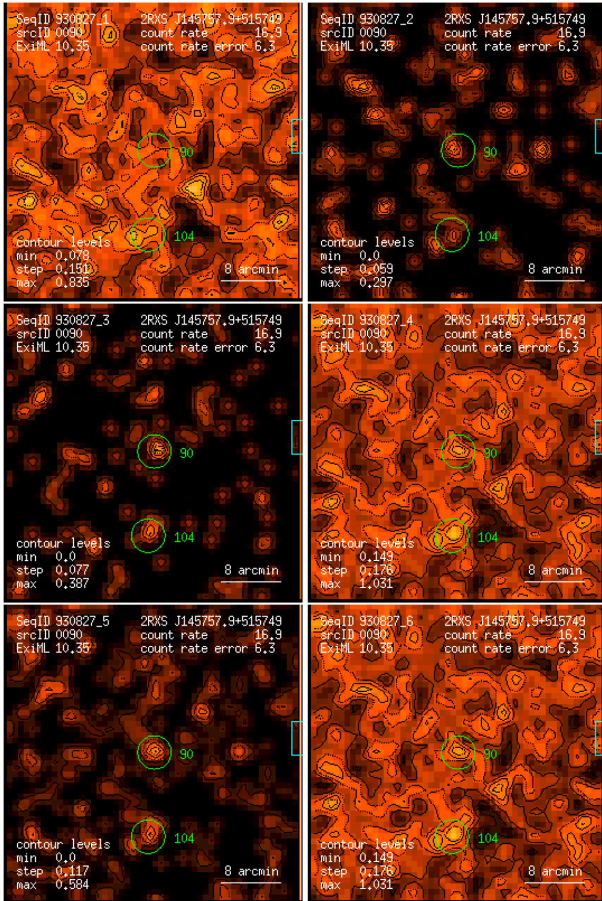
Figure 90: RASS 930827: detection 0090: band rate images, Gaussian filter: (1) PSPC channels 11 – 41, (2) 52 – 90, (3) 91 – 201, (4) 11 – 235, (5) 52 – 201, (6) 11 – 201. Broad band rates in counts/ks. Band rate contour levels in counts/ks/arcmin 2 .
