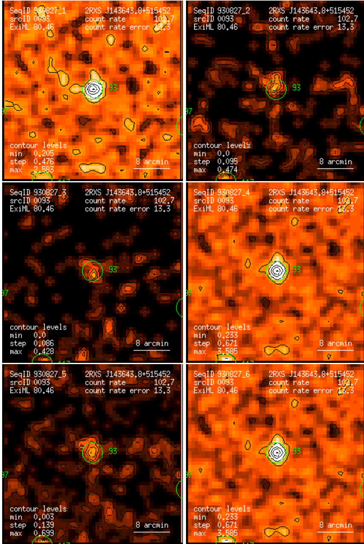
Figure 93: RASS 930827: detection 0093: band rate images, Gaussian filter: (1) PSPC channels 11 – 41, (2) 52 – 90, (3) 91 – 201, (4) 11 – 235, (5) 52 – 201, (6) 11 – 201. Broad band rates in counts/ks. Band rate contour levels in counts/ks/arcmin 2 .
