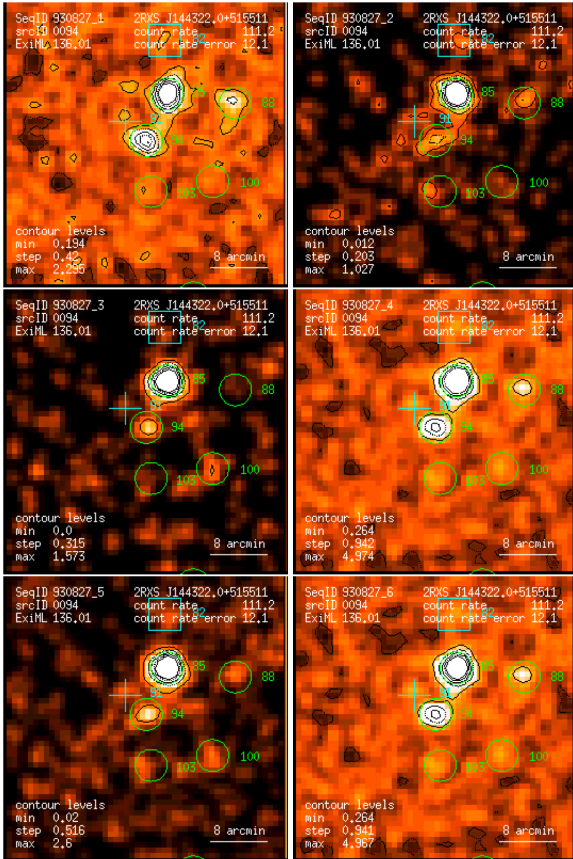
Figure 94: RASS 930827: detection 0094: band rate images, Gaussian filter: (1) PSPC channels 11 – 41, (2) 52 – 90, (3) 91 – 201, (4) 11 – 235, (5) 52 – 201, (6) 11 – 201. Broad band rates in counts/ks. Band rate contour levels in counts/ks/arcmin 2 .
