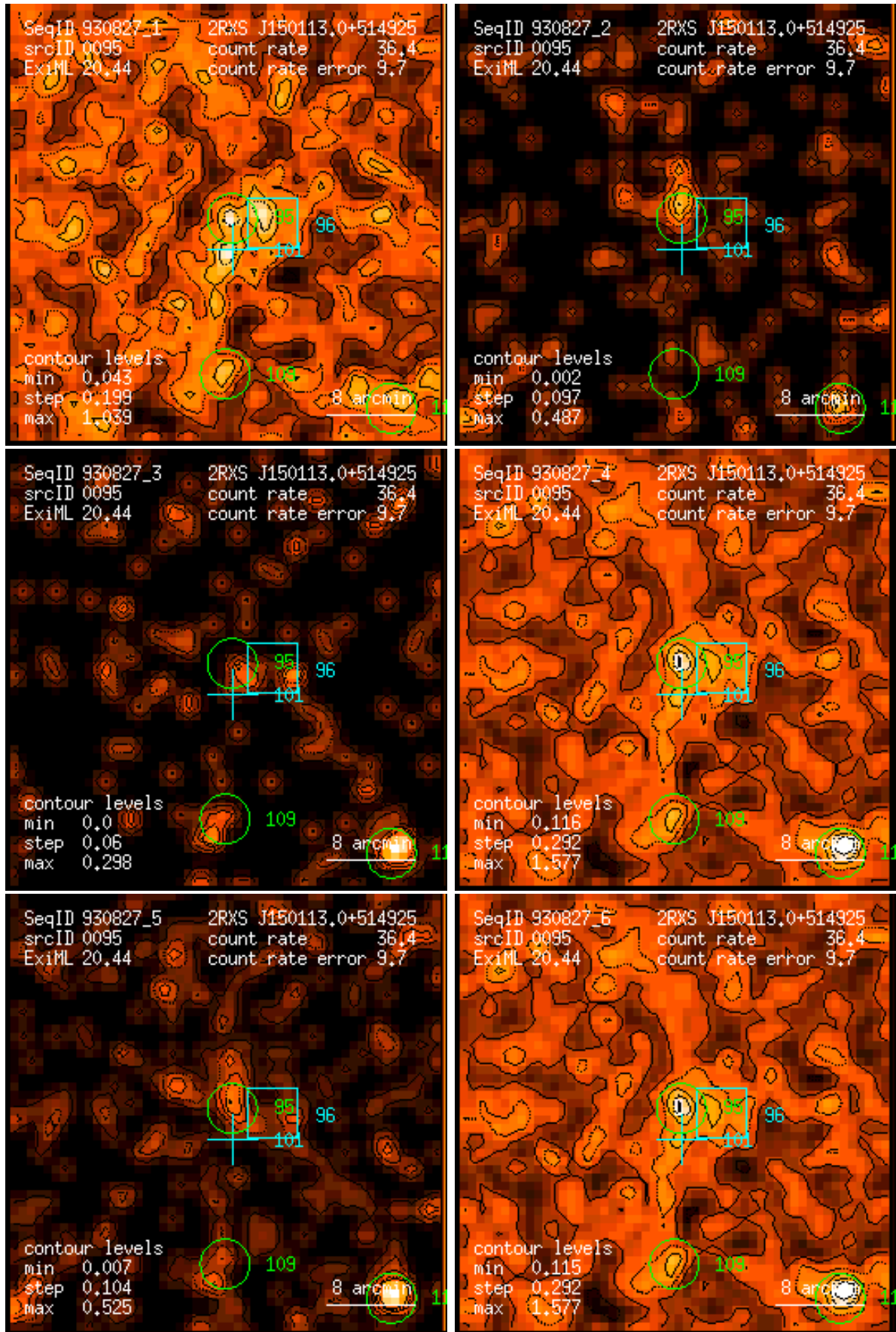
Figure 95: RASS 930827: detection 0095: band rate images, Gaussian filter: (1) PSPC channels 11 – 41, (2) 52 – 90, (3) 91 – 201, (4) 11 – 235, (5) 52 – 201, (6) 11 – 201. Broad band rates in counts/ks. Band rate contour levels in counts/ks/arcmin 2 .
