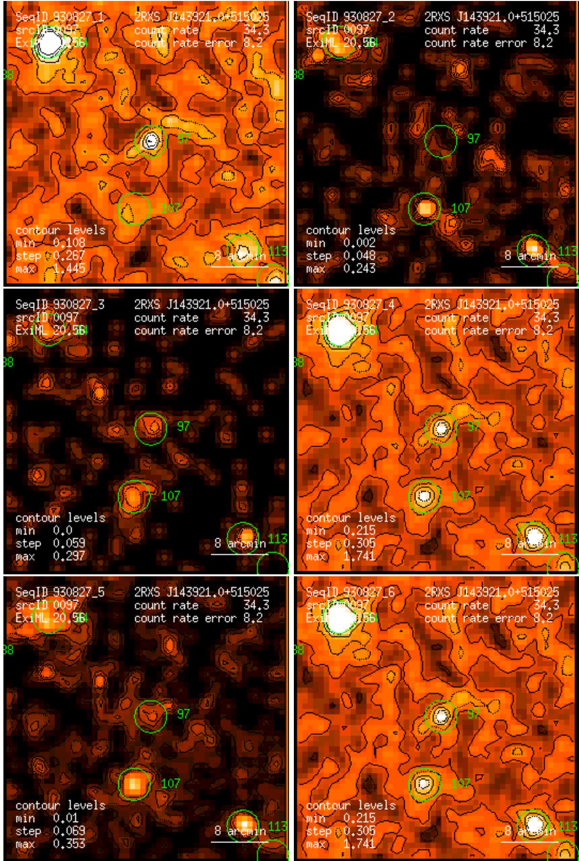
Figure 97: RASS 930827: detection 0097: band rate images, Gaussian filter: (1) PSPC channels 11 – 41, (2) 52 – 90, (3) 91 – 201, (4) 11 – 235, (5) 52 – 201, (6) 11 – 201. Broad band rates in counts/ks. Band rate contour levels in counts/ks/arcmin 2 .
