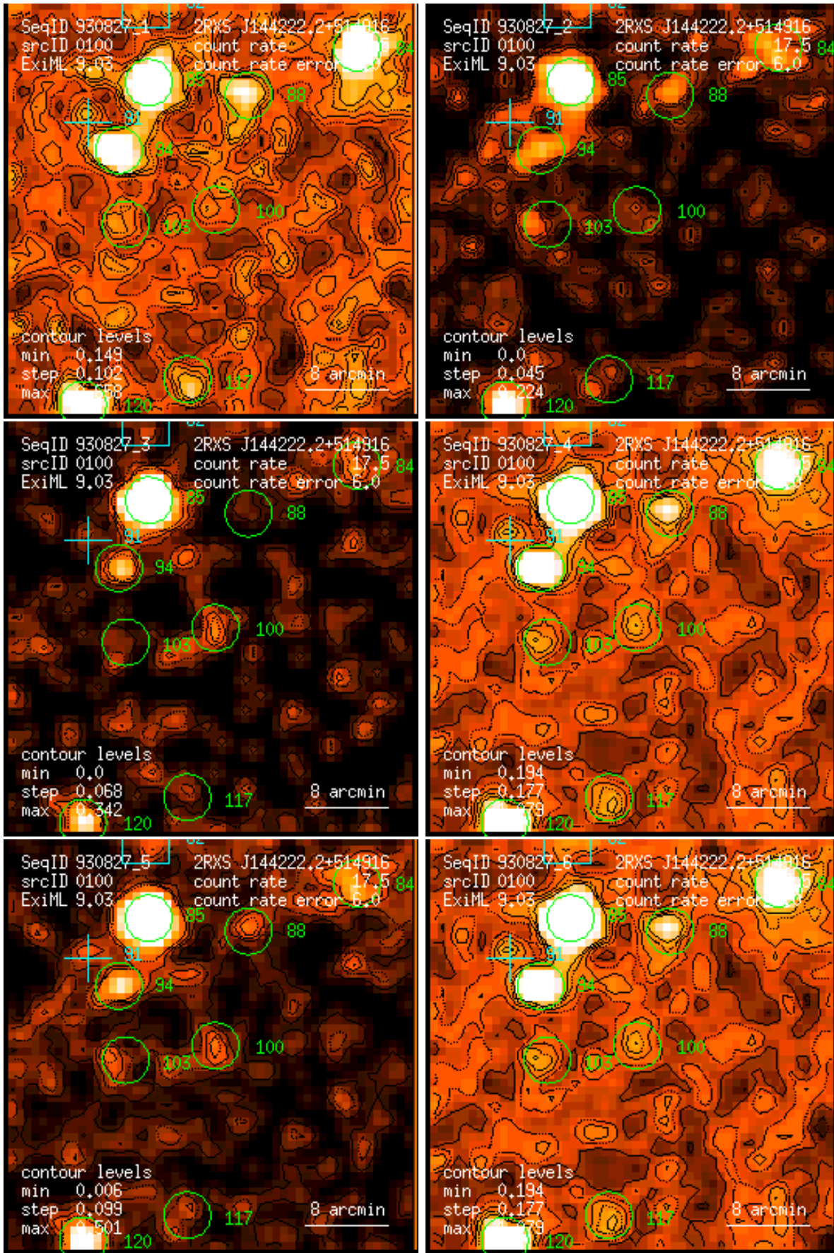
Figure 100: RASS 930827: detection 0100: band rate images, Gaussian filter: (1) PSPC channels 11 – 41, (2) 52 – 90, (3) 91 – 201, (4) 11 – 235, (5) 52 – 201, (6) 11 – 201. Broad band rates in counts/ks. Band rate contour levels in counts/ks/arcmin 2 .
