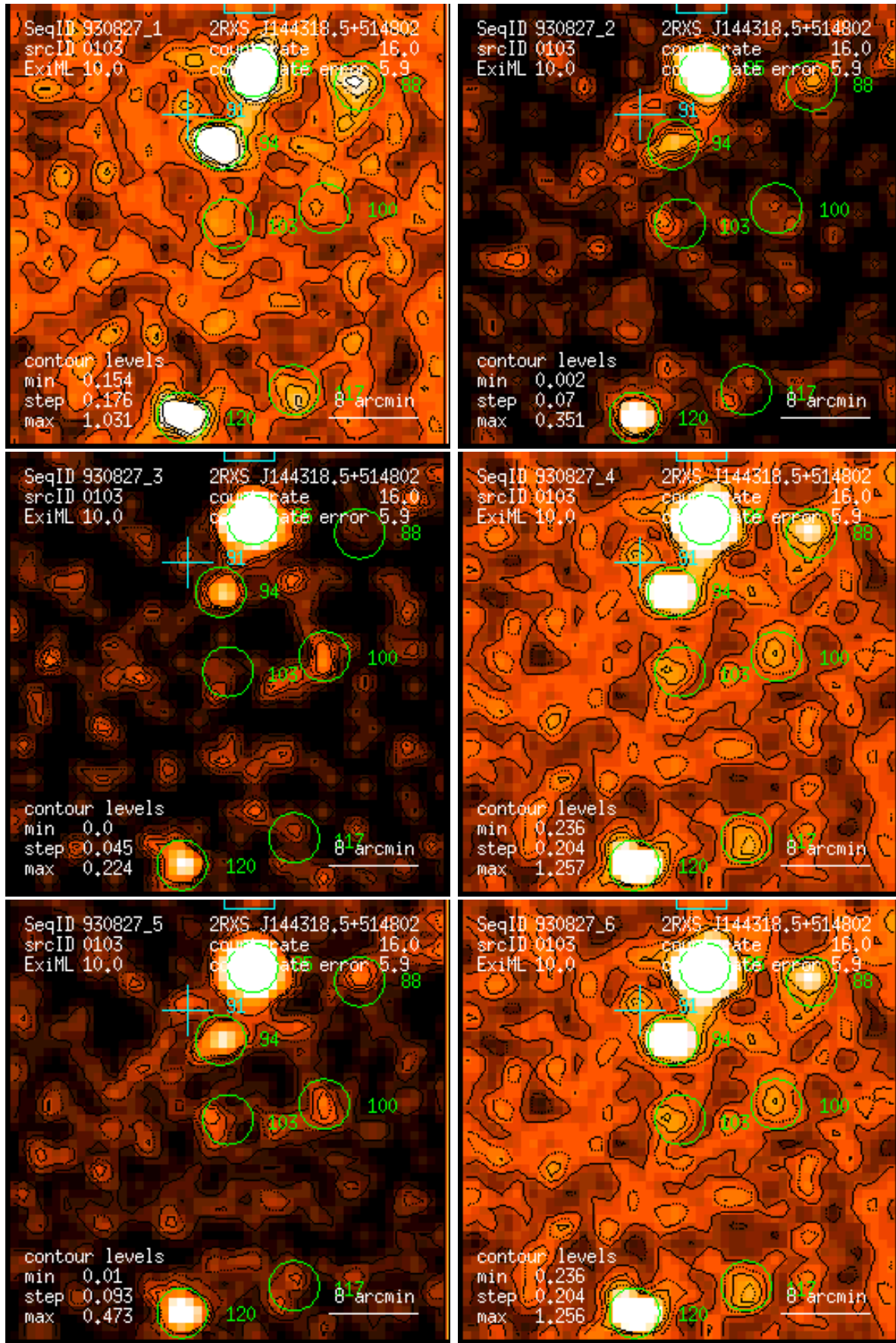
Figure 103: RASS 930827: detection 0103: band rate images, Gaussian filter: (1) PSPC channels 11 – 41, (2) 52 – 90, (3) 91 – 201, (4) 11 – 235, (5) 52 – 201, (6) 11 – 201. Broad band rates in counts/ks. Band rate contour levels in counts/ks/arcmin 2 .
