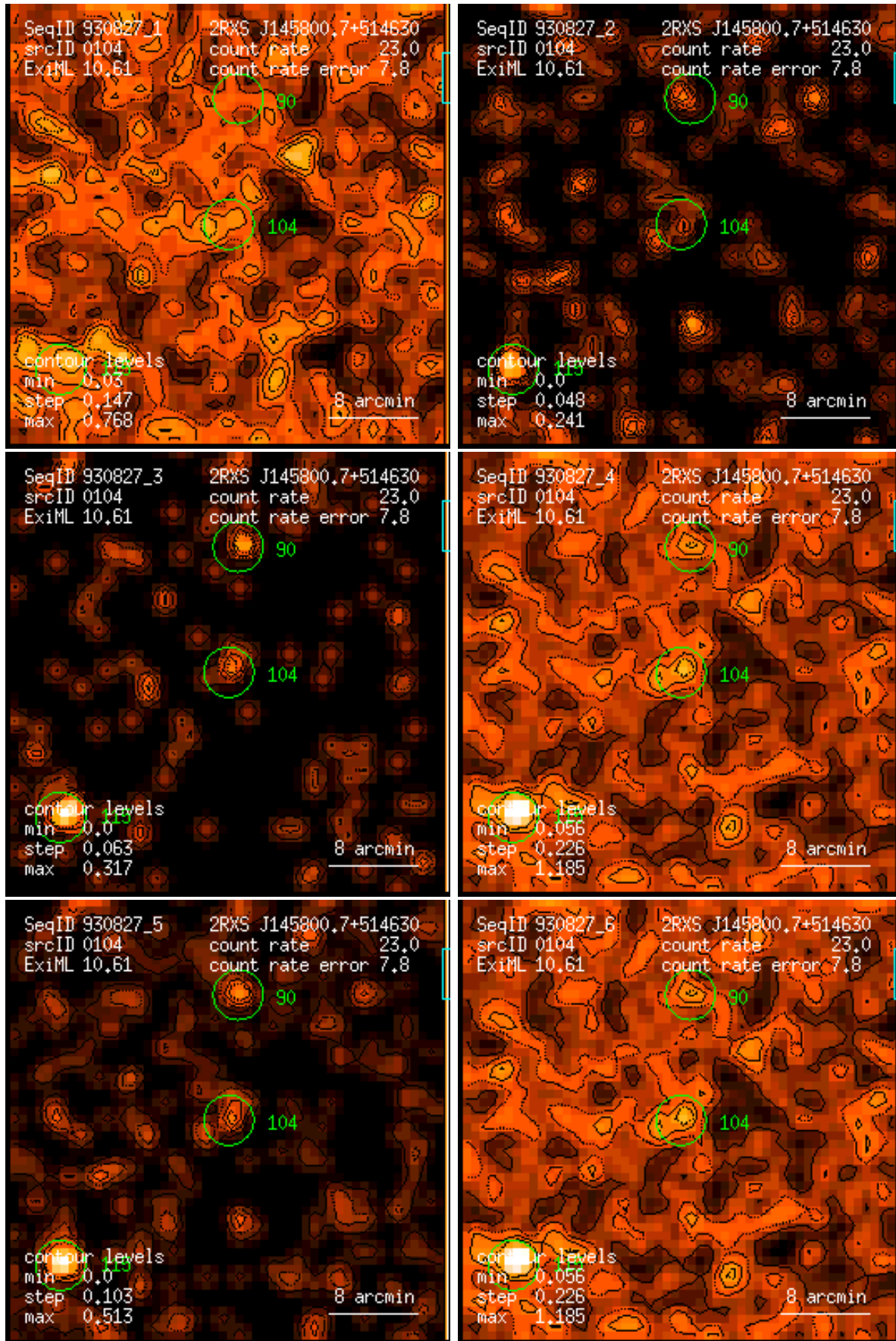
Figure 104: RASS 930827: detection 0104: band rate images, Gaussian filter: (1) PSPC channels 11 – 41, (2) 52 – 90, (3) 91 – 201, (4) 11 – 235, (5) 52 – 201, (6) 11 – 201. Broad band rates in counts/ks. Band rate contour levels in counts/ks/arcmin 2 .
