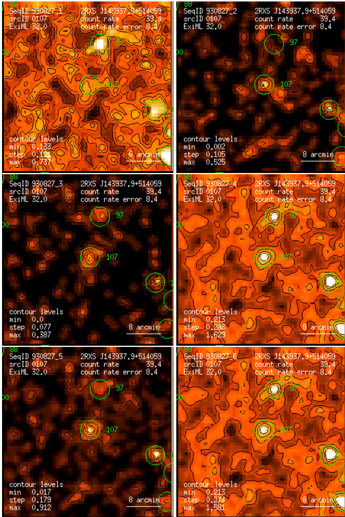
Figure 107: RASS 930827: detection 0107: band rate images, Gaussian filter: (1) PSPC channels 11 – 41, (2) 52 – 90, (3) 91 – 201, (4) 11 – 235, (5) 52 – 201, (6) 11 – 201. Broad band rates in counts/ks. Band rate contour levels in counts/ks/arcmin 2 .
