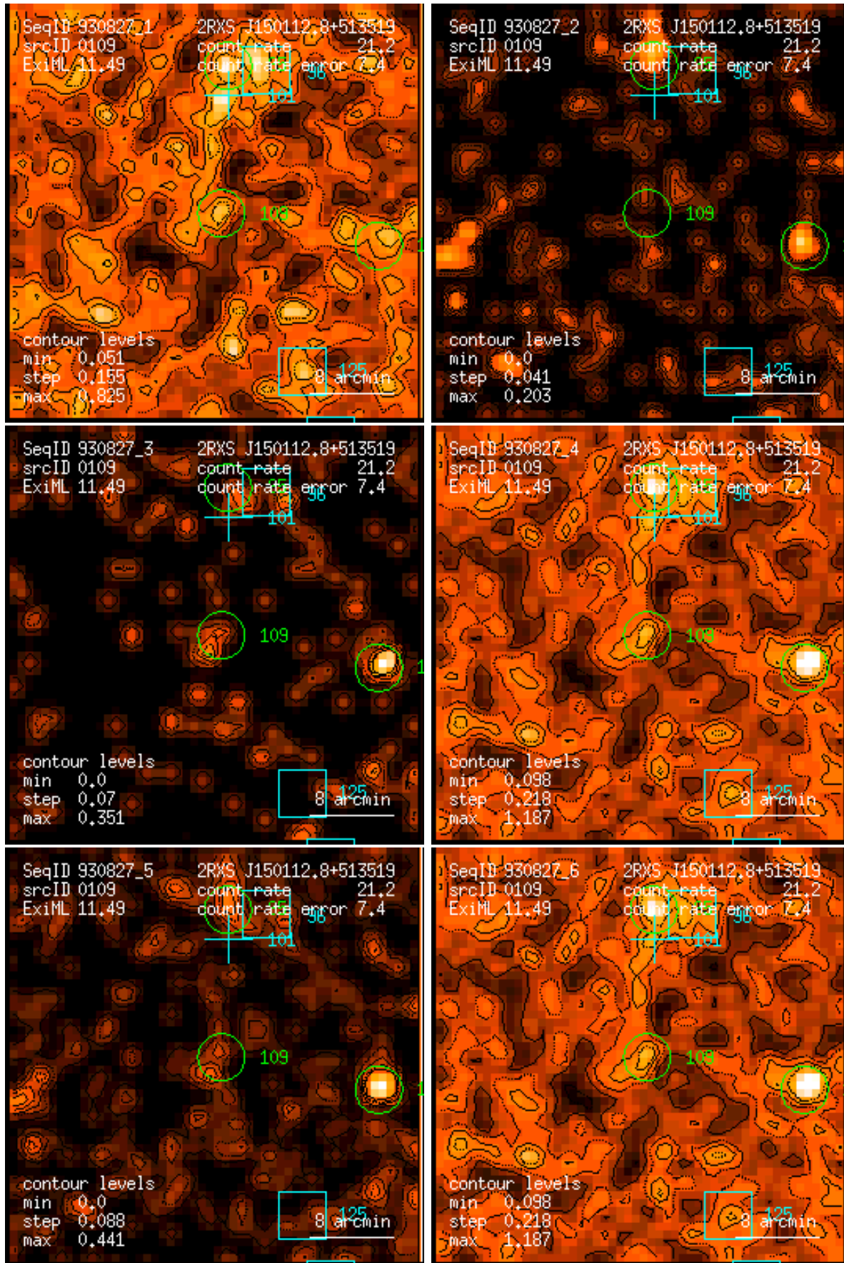
Figure 109: RASS 930827: detection 0109: band rate images, Gaussian filter: (1) PSPC channels 11 – 41, (2) 52 – 90, (3) 91 – 201, (4) 11 – 235, (5) 52 – 201, (6) 11 – 201. Broad band rates in counts/ks. Band rate contour levels in counts/ks/arcmin 2 .
