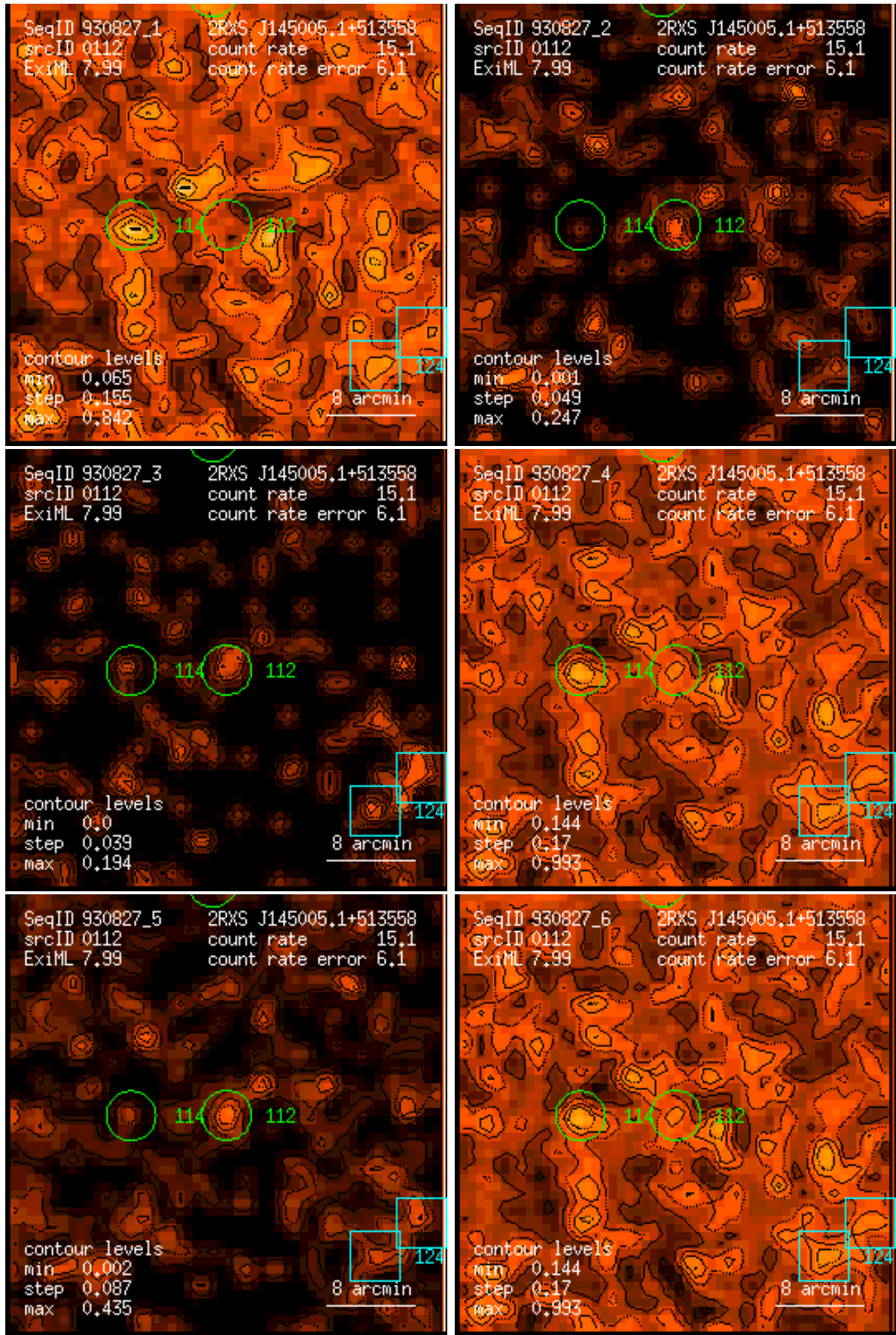
Figure 112: RASS 930827: detection 0112: band rate images, Gaussian filter: (1) PSPC channels 11 – 41, (2) 52 – 90, (3) 91 – 201, (4) 11 – 235, (5) 52 – 201, (6) 11 – 201. Broad band rates in counts/ks. Band rate contour levels in counts/ks/arcmin 2 .
