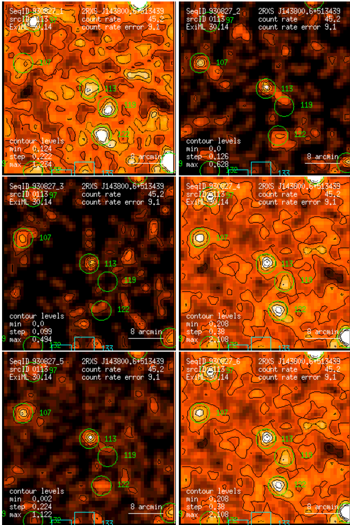
Figure 113: RASS 930827: detection 0113: band rate images, Gaussian filter: (1) PSPC channels 11 – 41, (2) 52 – 90, (3) 91 – 201, (4) 11 – 235, (5) 52 – 201, (6) 11 – 201. Broad band rates in counts/ks. Band rate contour levels in counts/ks/arcmin 2 .
