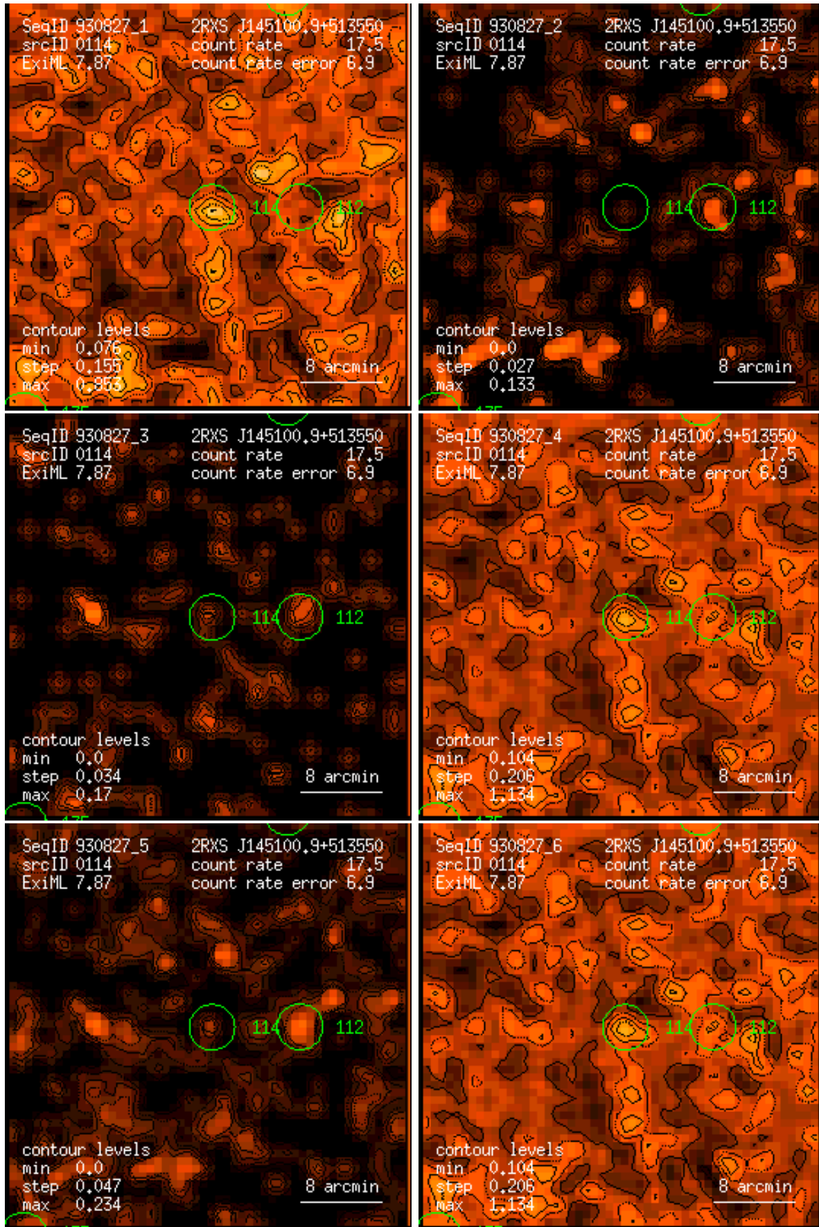
Figure 114: RASS 930827: detection 0114: band rate images, Gaussian filter: (1) PSPC channels 11 – 41, (2) 52 – 90, (3) 91 – 201, (4) 11 – 235, (5) 52 – 201, (6) 11 – 201. Broad band rates in counts/ks. Band rate contour levels in counts/ks/arcmin 2 .
