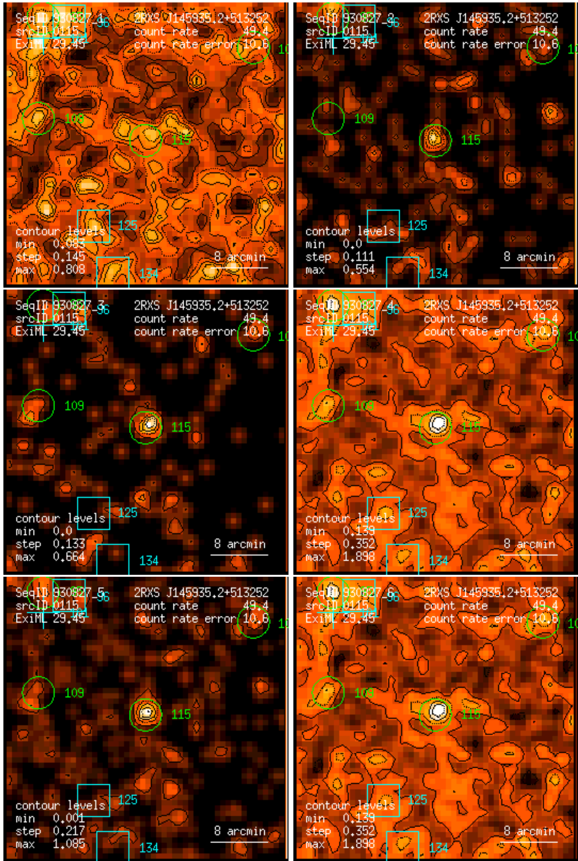
Figure 115: RASS 930827: detection 0115: band rate images, Gaussian filter: (1) PSPC channels 11 – 41, (2) 52 – 90, (3) 91 – 201, (4) 11 – 235, (5) 52 – 201, (6) 11 – 201. Broad band rates in counts/ks. Band rate contour levels in counts/ks/arcmin 2 .
