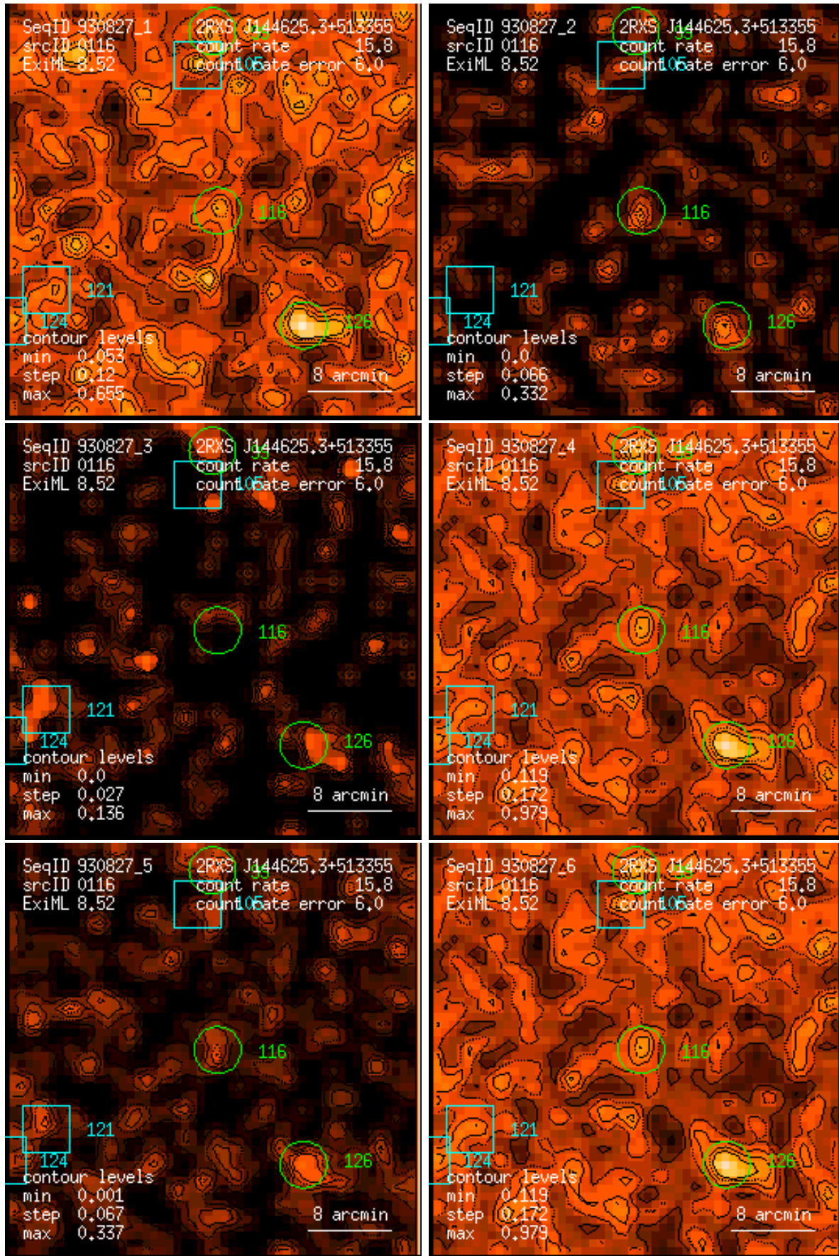
Figure 116: RASS 930827: detection 0116: band rate images, Gaussian filter: (1) PSPC channels 11 – 41, (2) 52 – 90, (3) 91 – 201, (4) 11 – 235, (5) 52 – 201, (6) 11 – 201. Broad band rates in counts/ks. Band rate contour levels in counts/ks/arcmin 2 .
