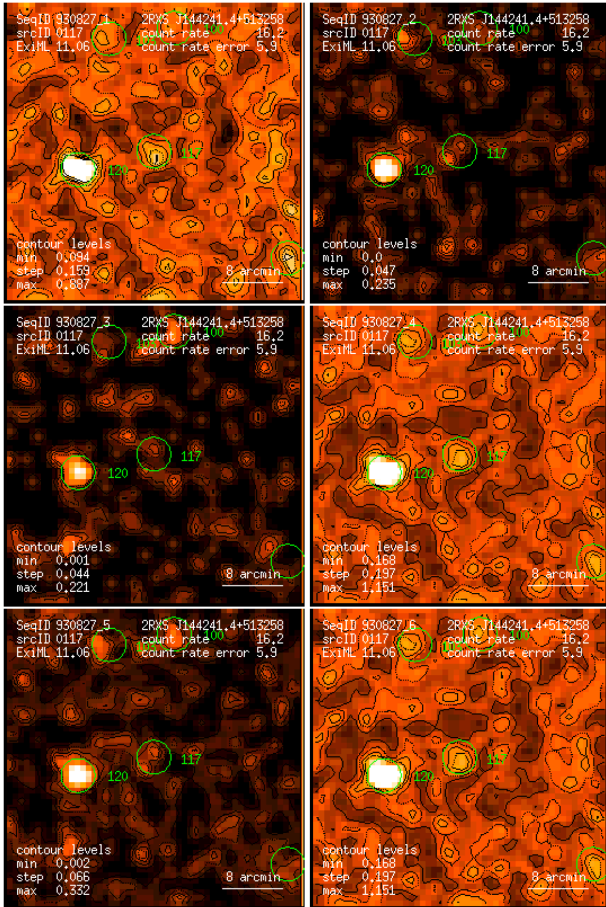
Figure 117: RASS 930827: detection 0117: band rate images, Gaussian filter: (1) PSPC channels 11 – 41, (2) 52 – 90, (3) 91 – 201, (4) 11 – 235, (5) 52 – 201, (6) 11 – 201. Broad band rates in counts/ks. Band rate contour levels in counts/ks/arcmin 2 .
