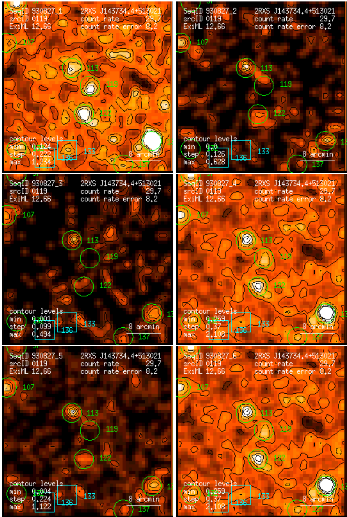
Figure 119: RASS 930827: detection 0119: band rate images, Gaussian filter: (1) PSPC channels 11 – 41, (2) 52 – 90, (3) 91 – 201, (4) 11 – 235, (5) 52 – 201, (6) 11 – 201. Broad band rates in counts/ks. Band rate contour levels in counts/ks/arcmin 2 .
