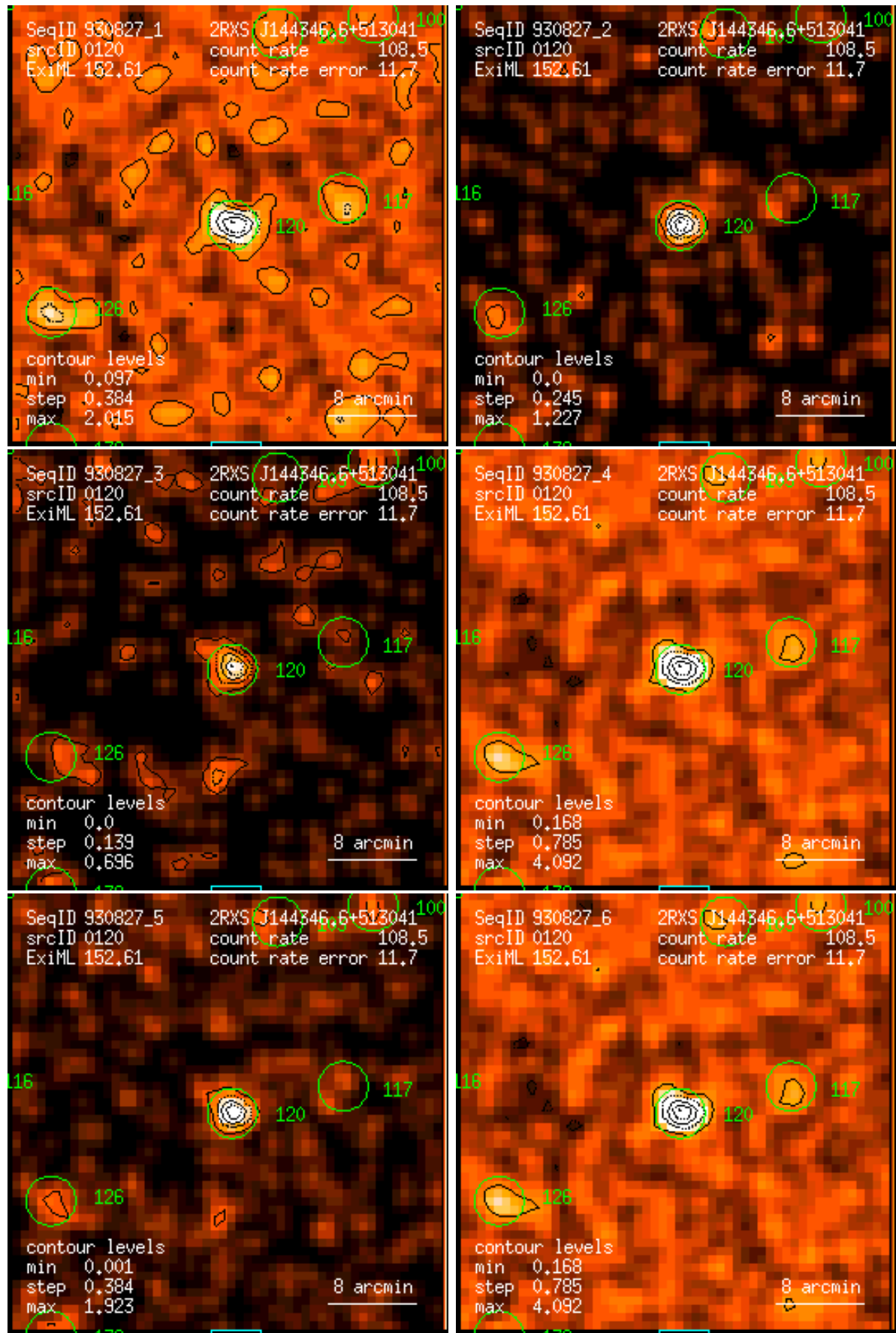
Figure 120: RASS 930827: detection 0120: band rate images, Gaussian filter: (1) PSPC channels 11 – 41, (2) 52 – 90, (3) 91 – 201, (4) 11 – 235, (5) 52 – 201, (6) 11 – 201. Broad band rates in counts/ks. Band rate contour levels in counts/ks/arcmin 2 .
