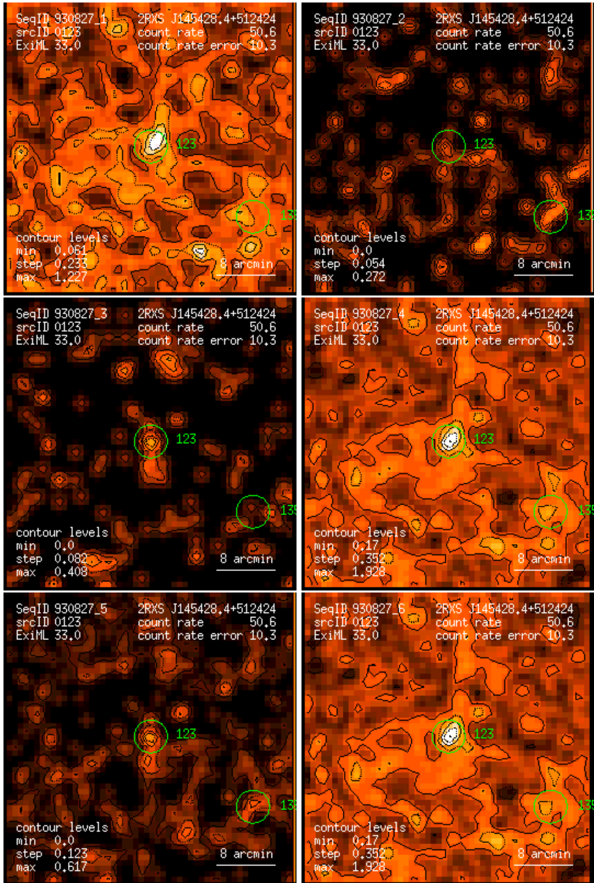
Figure 123: RASS 930827: detection 0123: band rate images, Gaussian filter: (1) PSPC channels 11 – 41, (2) 52 – 90, (3) 91 – 201, (4) 11 – 235, (5) 52 – 201, (6) 11 – 201. Broad band rates in counts/ks. Band rate contour levels in counts/ks/arcmin 2 .
