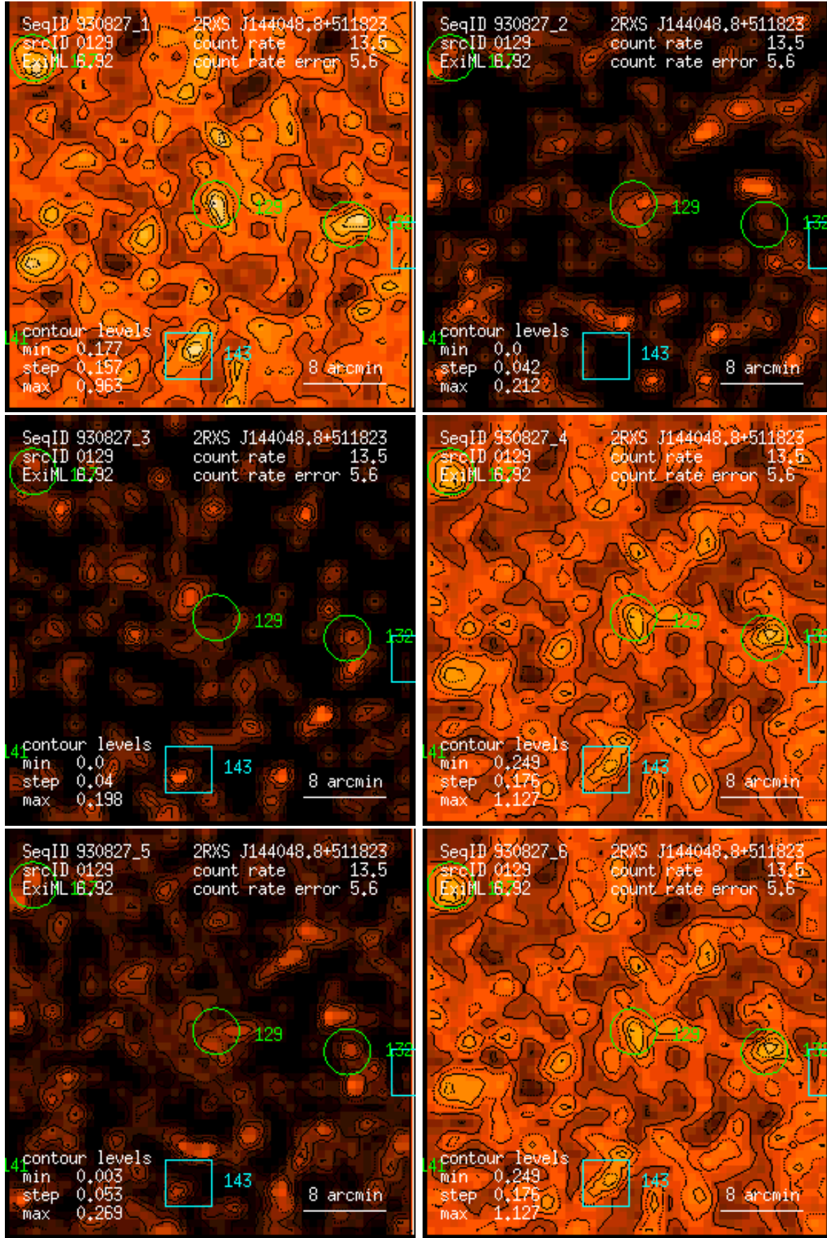
Figure 129: RASS 930827: detection 0129: band rate images, Gaussian filter: (1) PSPC channels 11 – 41, (2) 52 – 90, (3) 91 – 201, (4) 11 – 235, (5) 52 – 201, (6) 11 – 201. Broad band rates in counts/ks. Band rate contour levels in counts/ks/arcmin 2 .
