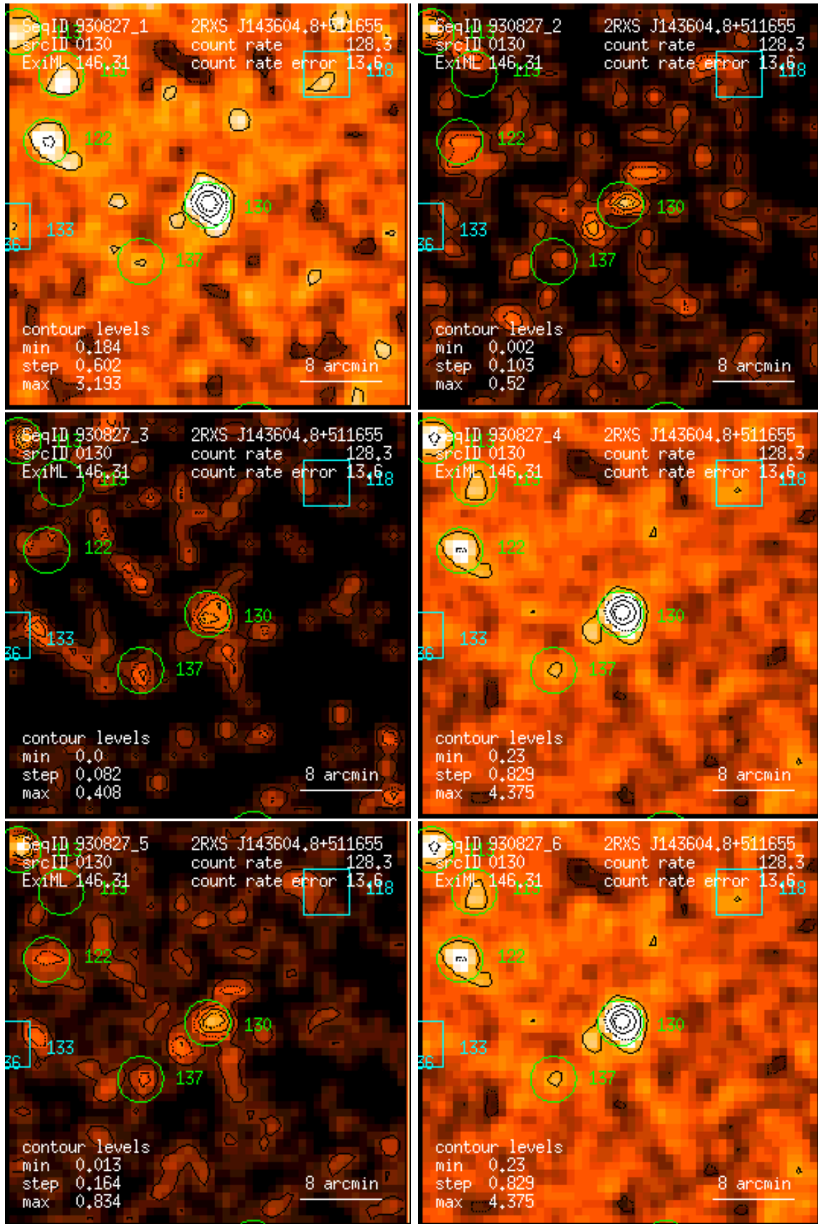
Figure 130: RASS 930827: detection 0130: band rate images, Gaussian filter: (1) PSPC channels 11 – 41, (2) 52 – 90, (3) 91 – 201, (4) 11 – 235, (5) 52 – 201, (6) 11 – 201. Broad band rates in counts/ks. Band rate contour levels in counts/ks/arcmin 2 .
