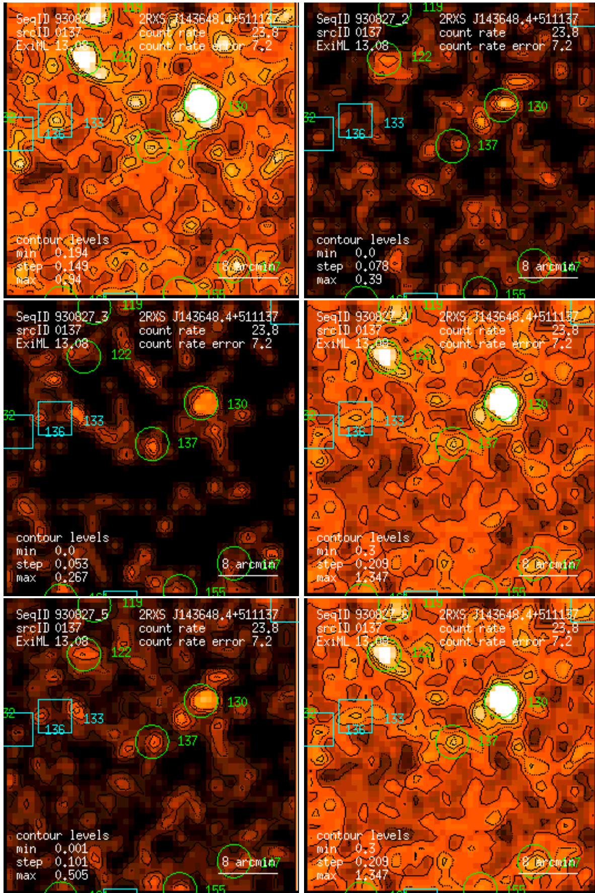
Figure 137: RASS 930827: detection 0137: band rate images, Gaussian filter: (1) PSPC channels 11 – 41, (2) 52 – 90, (3) 91 – 201, (4) 11 – 235, (5) 52 – 201, (6) 11 – 201. Broad band rates in counts/ks. Band rate contour levels in counts/ks/arcmin 2 .
