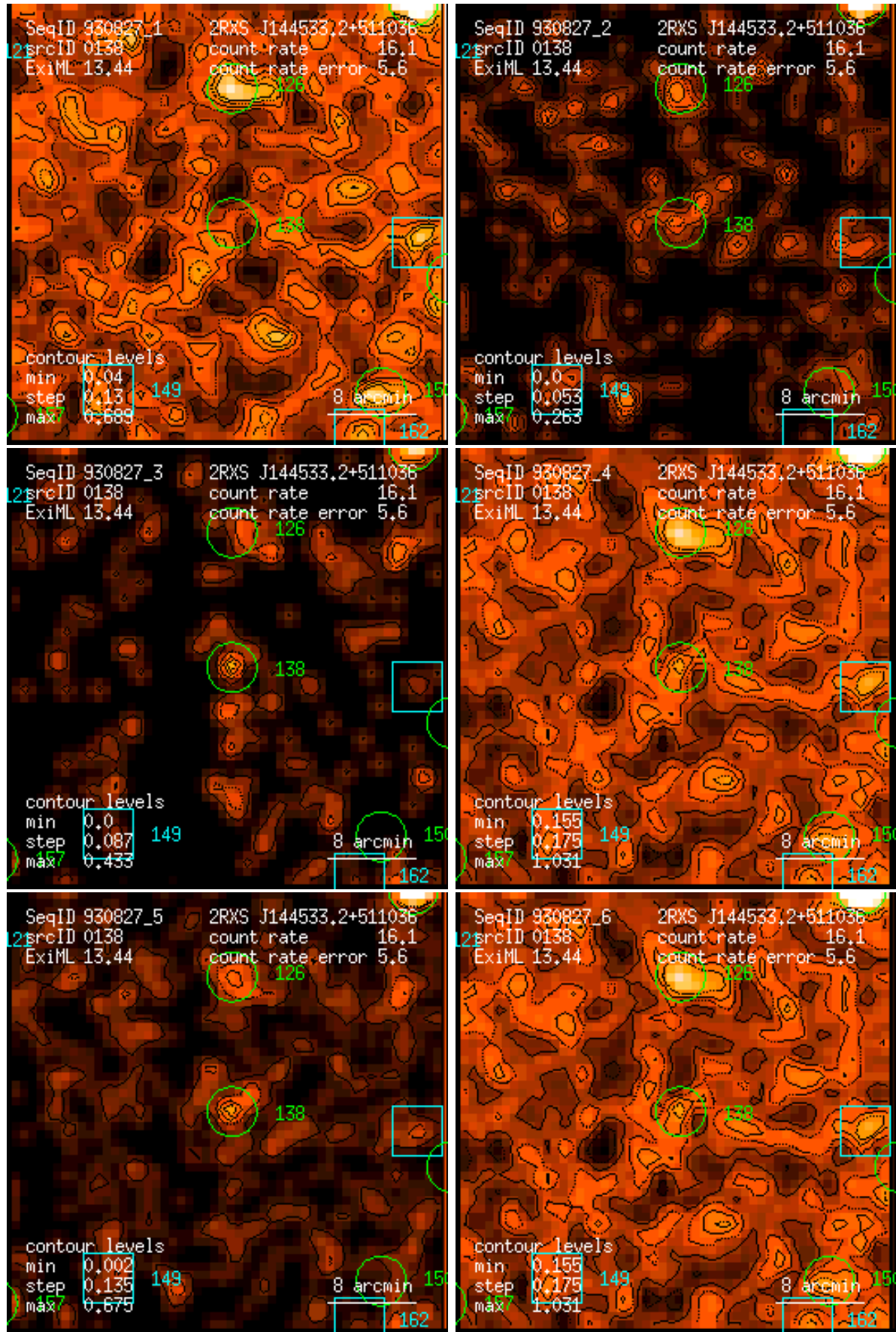
Figure 138: RASS 930827: detection 0138: band rate images, Gaussian filter: (1) PSPC channels 11 – 41, (2) 52 – 90, (3) 91 – 201, (4) 11 – 235, (5) 52 – 201, (6) 11 – 201. Broad band rates in counts/ks. Band rate contour levels in counts/ks/arcmin 2 .
